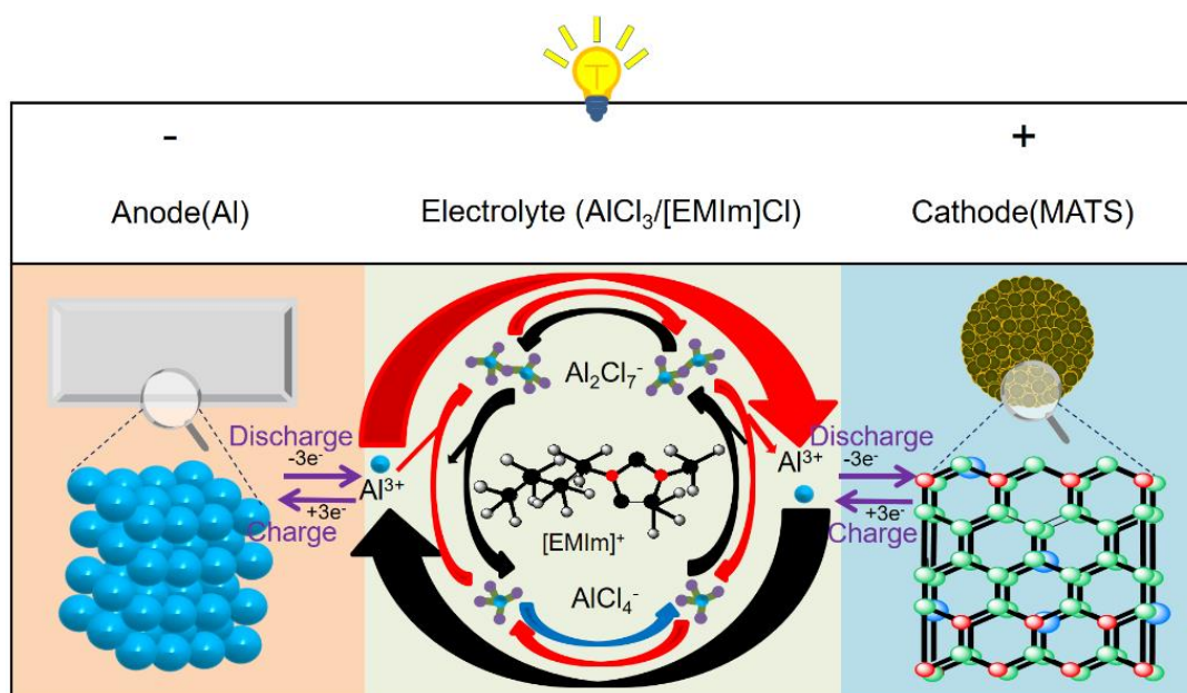
Scheme 1. Schematic illustration of the reaction mechanism of NAIBs with MATS cathode material and AlCl 3 /[EMIm]Cl electrolyte.
