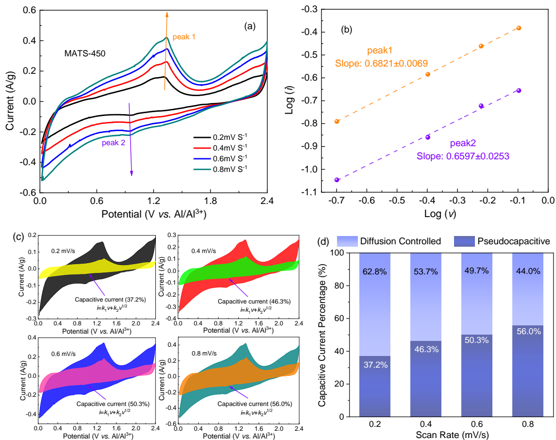
Figure 6. The CV curves at various scan rates and their derived pseudocapacitive analysis of the MATS-450: (a) CV curves at 0.2-0.8 mV s -1 ; (b) their linear relationship between log ( i )-log ( v ); and (c) their contribution ratio of the capacitive capacities and diffusion-limited capacities and (d) the corresponding bar diagram.
