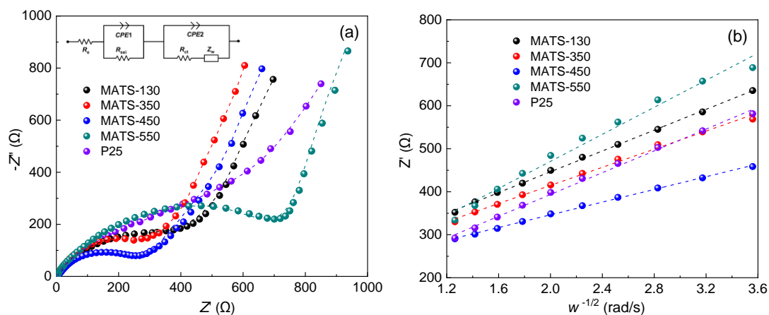
Figure 4. (a) The Nyquist plots and their fitting results (dotted lines) after three cycles with their equivalent circuit (inset); (b) the relationship between Z' and \omega^{-1/2} for the MATS and P25 cathodes of NAIBs.
