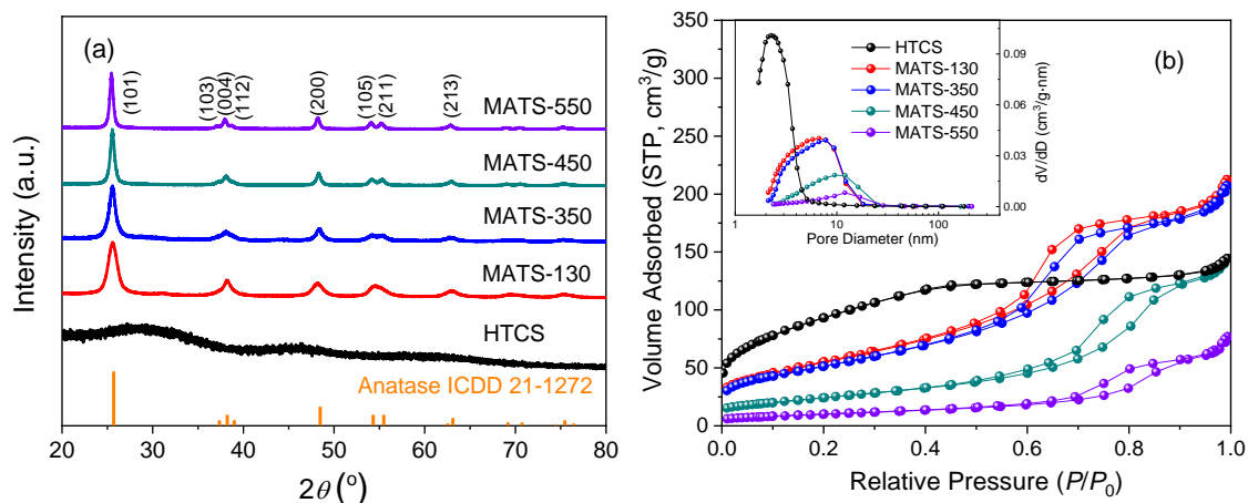
Figure 1. (a) XRD patterns and (b) N 2 adsorption and desorption isotherms and the pore size distributions obtained from the desorption branches (inset) of HTCS and their MATS products upon the microwave-assisted hydrothermal process at 130 °C (MATS-130) followed with annealing at 350–550 °C (MATS-350-550).
