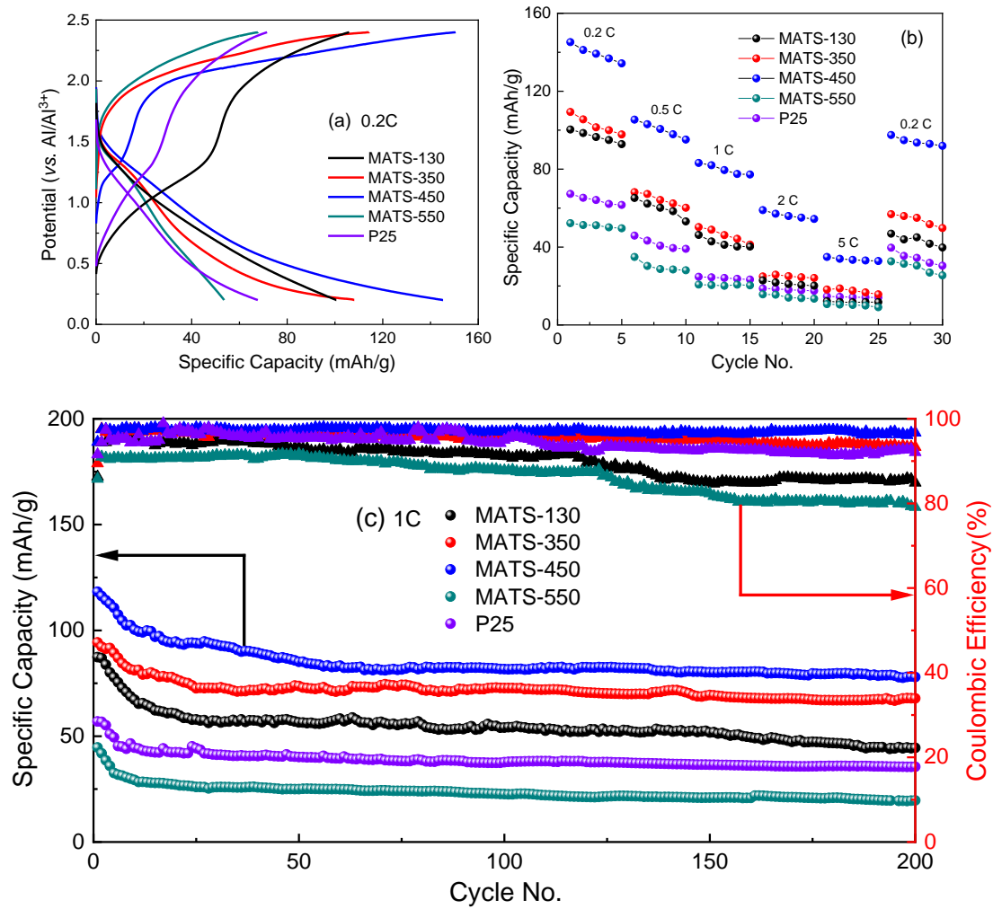
Figure 3. (a) Initial charge-discharge curves at 0.2C, (b) rate capability, and (c) cycling performances at 1 C of P25 and the different MATS samples in the range of 0.2–2.4 V (vs. Al/Al 3+ ).
