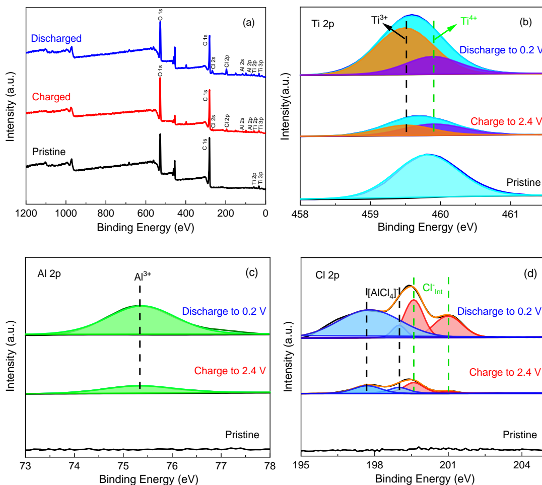
Figure 8. (a) Ex-situ XPS survey of pristine (black), charged (red), and discharged (blue) MATS-450 cathodes after 50 cycles, and their corresponding high-resolution XPS spectra of (b) Ti 2p, (c) Al 2p, and (d) Cl 2p.
