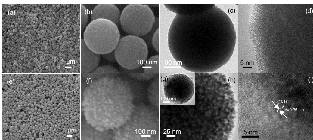
Figure 2. Comparative SEM and TEM micrographs at different magnifications of (a-d) HTCS and (e-i) MATS-450.
