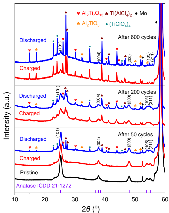
Figure 9. Ex-situ XRD patterns of pristine (black), charged (red), and discharged (blue) MTS-450 cathodes after 50, 200 and 600 cycles at 1 C between 0.2-2.4 V (vs. \text{Al}^{3+}/\text{Al} ).
