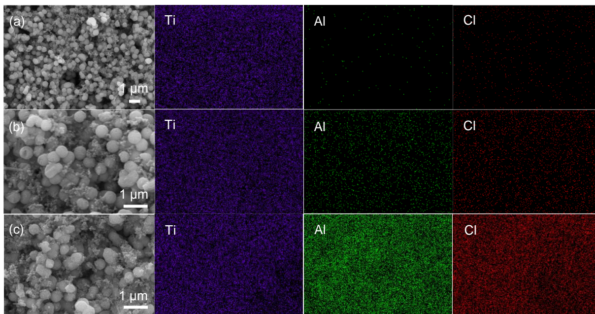
Figure 7. SEM micrographs with corresponding EDX elemental mappings of (a) pristine without cycling, (b) charged and (c) discharged MATS-450 cathodes obtained after 50 cycles.
