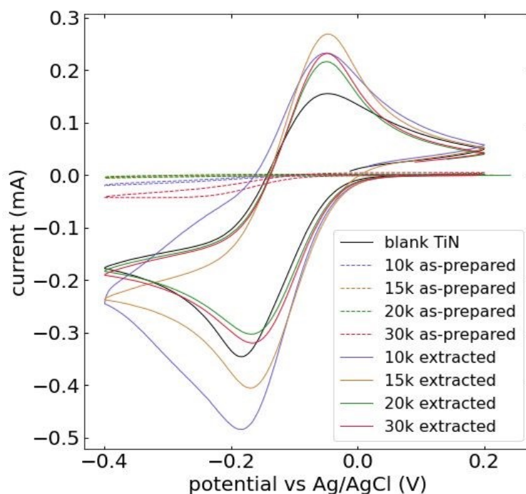
Figure 5: Cyclic voltammetry of mesoporous silica films (prepared at 100 Hz) on TiN in 5mM [\text{Ru}(\text{NH}_3)_6]\text{Cl}_3 with 0.1M \text{NaNO}_3 between -0.4 V and 0.2 V vs Ag/AgCl at a scan rate of 20 mV/s, one cycle each. Solid black line shows response of a blank TiN substrate with an electrode area of 5 x 15 mm. Coloured dashed lines show the current response before, solid ones after, surfactant removal.
