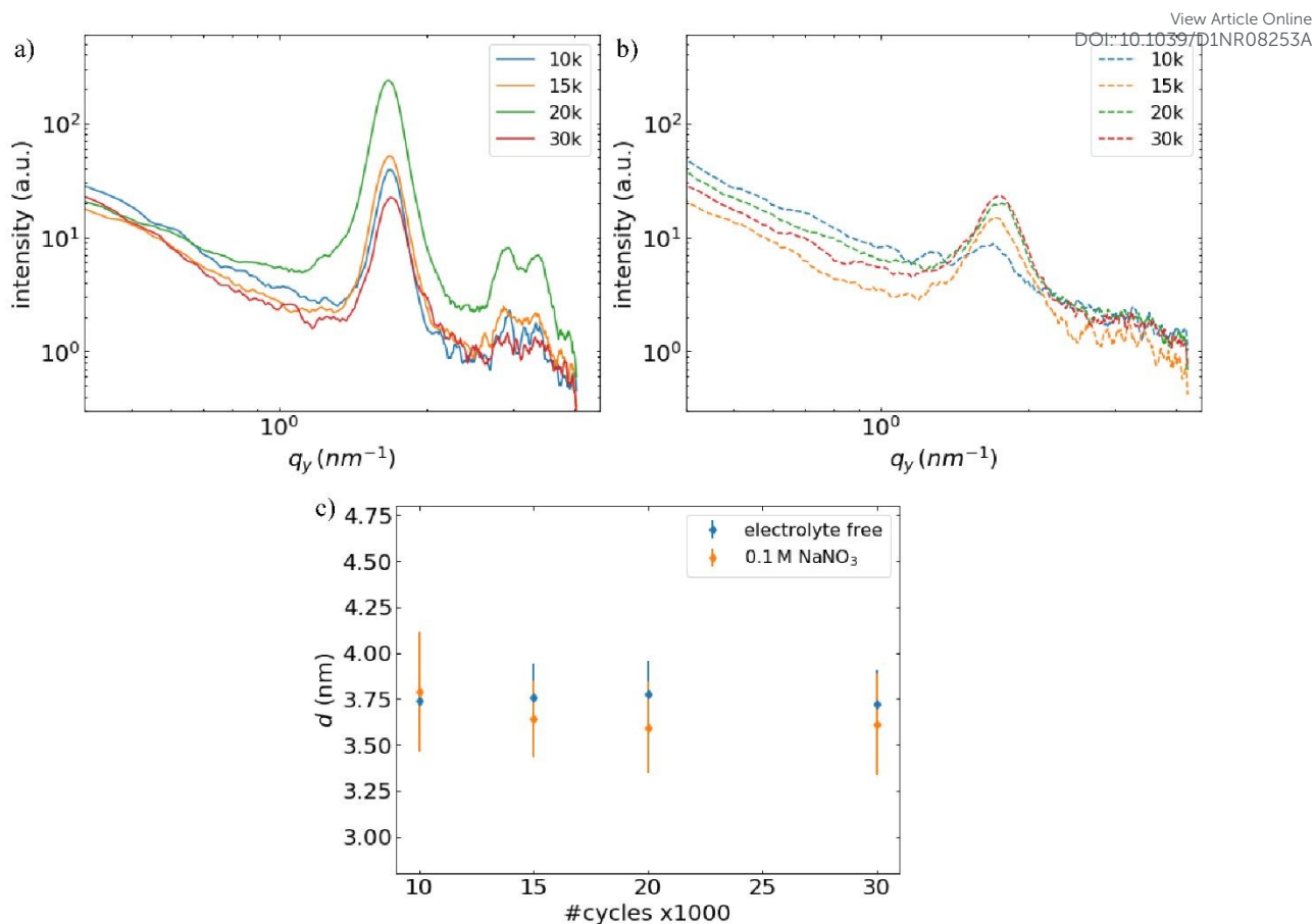
Figure 4: Horizontal scattering profiles for mesoporous silica films produced at 100 Hz, between -1.0 V and -2.0 V with a) electrolyte-free and b) 0.1 M NaNO 3 containing sol. c) Comparison of the d -spacings corresponding to the peaks shown in a) and b) calculated using d=2\pi/q .
