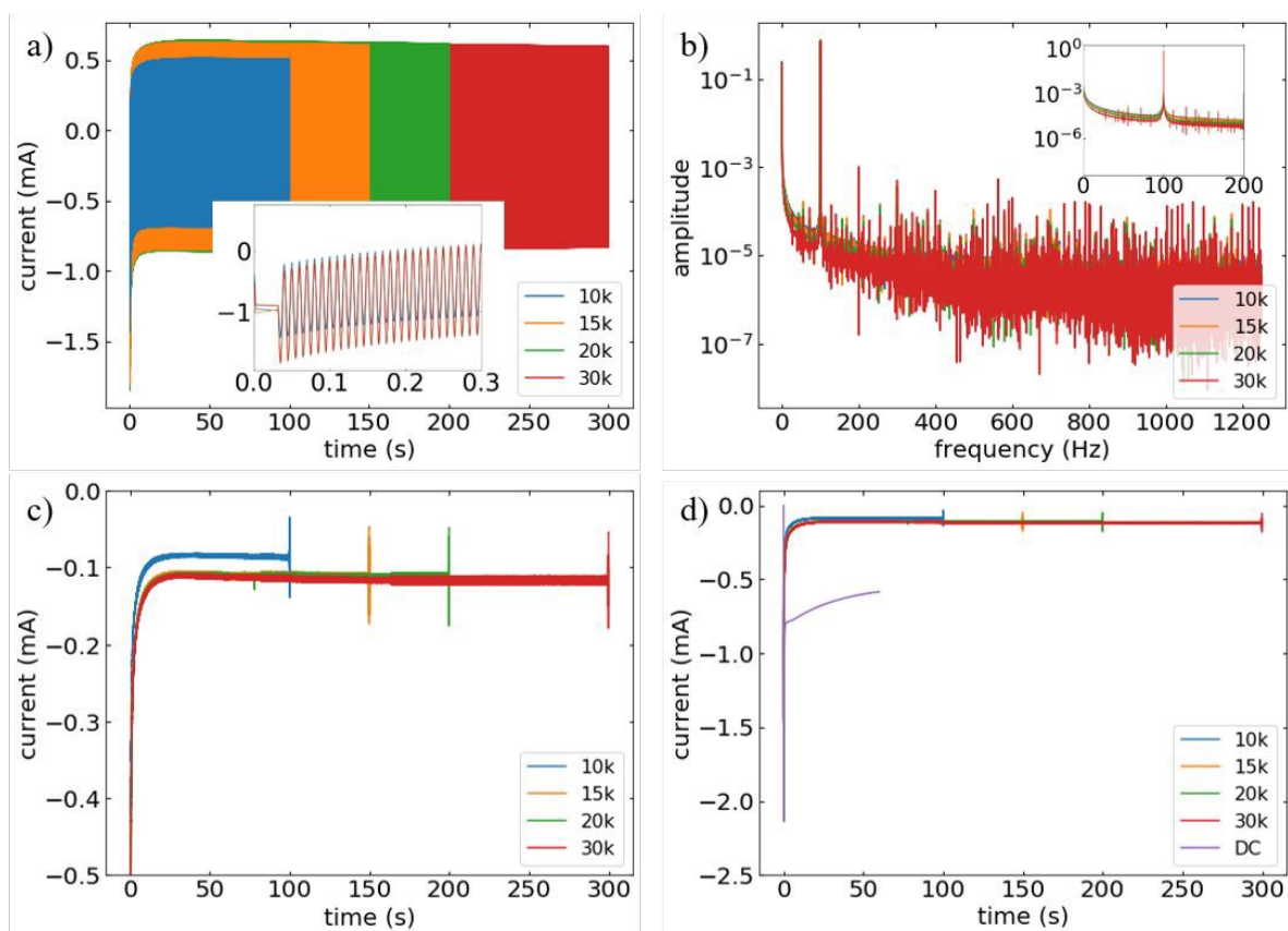
Figure 2: a) Raw currents recorded during the deposition of silica using a sinusoidal signal with a frequency of 100 Hz, between -1.0 V and -2.0 V with deposition times of 10,000, 15,000, 20,000, and 30,000 periods (100, 150, 200 and 300 s). Inset: zoomed plot of the same signals for the period between 0 and 0.3 s. b) Fourier-Transform of the data shown in a) produced using a custom-made python script. Inset: zoom to the range 0-200 Hz. c) Data from a) filtered using another custom python script which employs a band stop notch filter at 100 Hz with Q=30 . d) Same data as c) plotted in conjunction with a current transient obtained from a deposition at constant potential of -2.0 V (DC) for 60 s.
