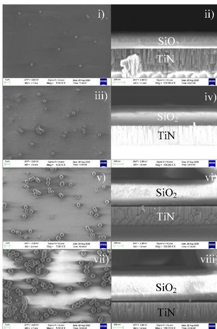
Figure 1: SEM images of mesoporous silica films deposited at 100 Hz, between -1.0 V and -2.0 V with deposition times of 10,000 periods ( i and ii ), 15,000 periods ( iii and iv ), 20,000 periods ( v and vi ) and 30,000 periods ( vii and viii ) of potential. The left-hand images are top-down and the right-hand cross-sections on cleaved samples.
