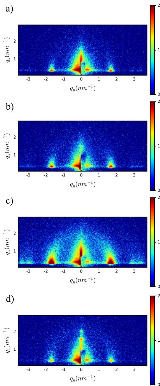
Figure 3: 2D GISAXS images measured with an incident angle of 0.3^\circ for a duration of 15 min for mesoporous silica samples deposited at 100 Hz, between -1.0 V and -2.0 V with deposition times of a) 10,000, b) 15,000, c) 20,000, and d) 30,000 periods.
