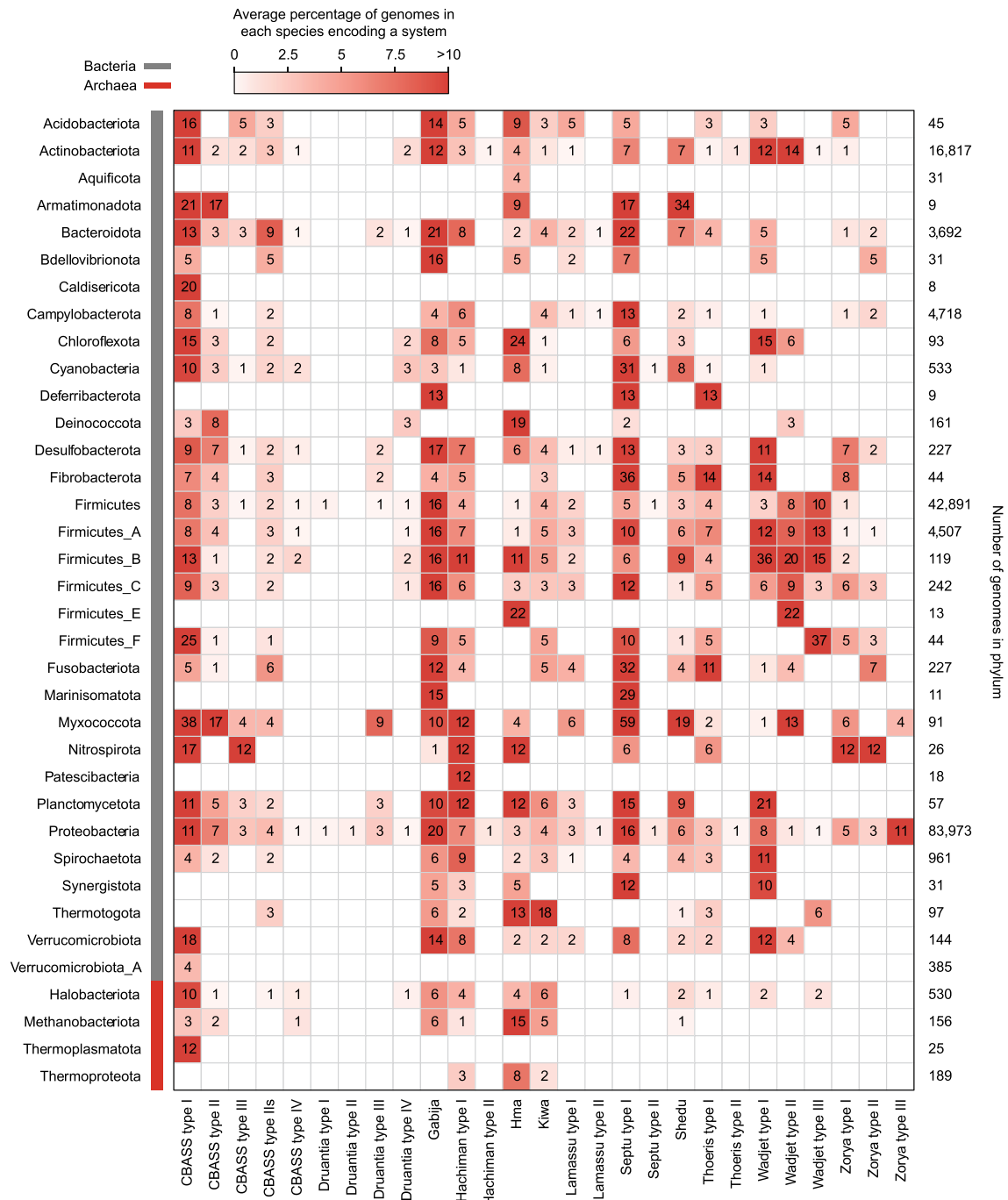
Figure 4. Abundance of defence systems identified with PADLOC in bacteria and archaea. All genomes from RefSeq v201 Archaea and Bacteria were searched with PADLOC. The values in the boxes represent, for each phylum, the average percentage of genomes in each species encoding a system, grouped using GTDB taxonomy (44); system prevalence is weighted in this way to limit biases in phyla that contain many closely related genomes of the same species. The colouring in each box provides a visual representation of these values. Shown are phyla with more than five genomes and at least one type of system. A species-level comparison is provided in Supplementary Figure S6 and the full data are provided in Supplementary Table S5.
