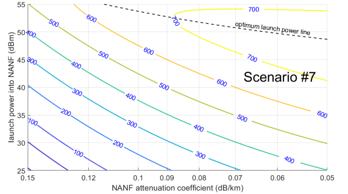
Fig. 7. Scenario #7. NANF system throughput isolines (Tb/s) over the plane (NANF loss, NANF launch power). The NANF systems operate over the 1450-1850 nm band (44.7 THz). Amplifierless single-span of 250 km. IMI is assumed absent or negligible. The receivers are assumed to operate with a 10 dB SNR penalty vs. the ideal value of Eq. (11).
