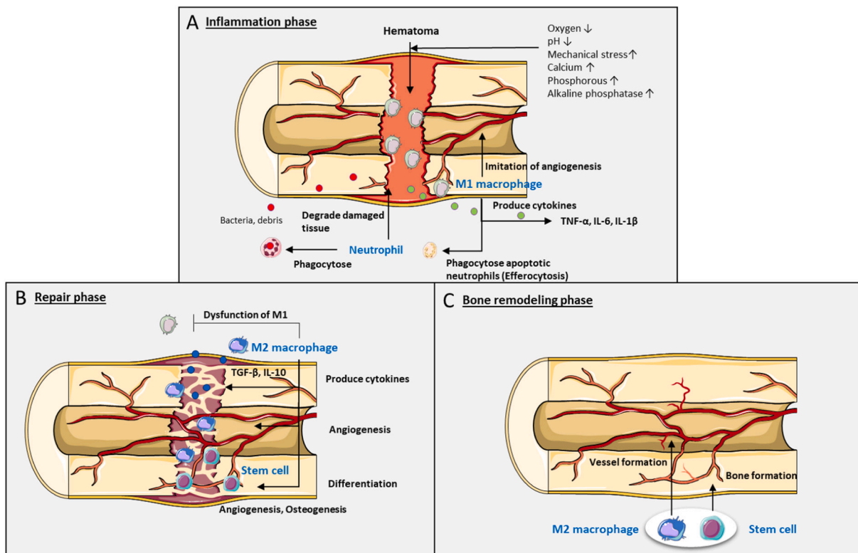
Fig. 2. A complex and well-orchestrated bone repair process involving three phases; inflammation, repair, and remodelling phases.
