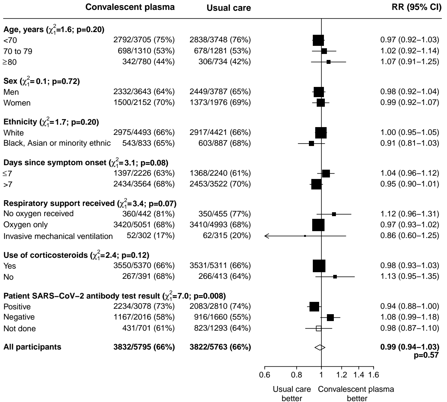
Webfigure 3: Discharged Alive within 28 Days, According to Subgroup
