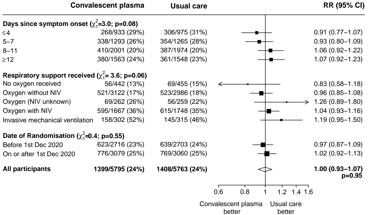
Webfigure 1: Mortality at 28 Days, According to Retrospectively-Defined Categories of Days Since Onset, Respiratory Support Received and Date of Randomisation
