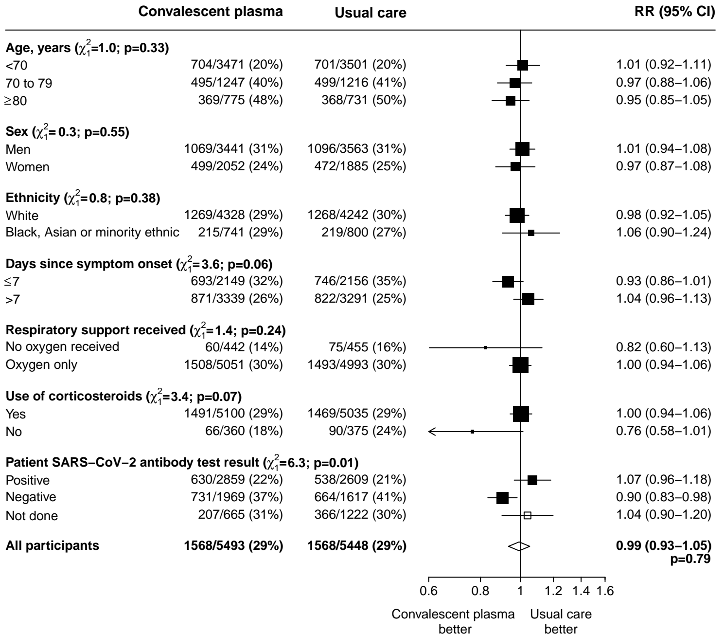
Webfigure 4: Invasive Mechanical Ventilation or Death, According to Subgroup
