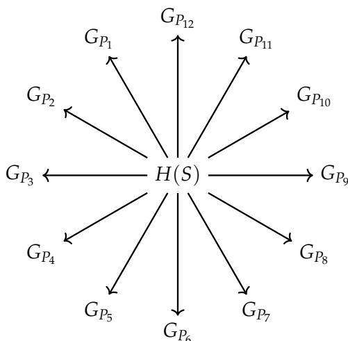
FIGURE 3.43: A graph of groups defining G(S) , each edge is assumed to be labelled H_{P_i} for the corresponding P_i .
