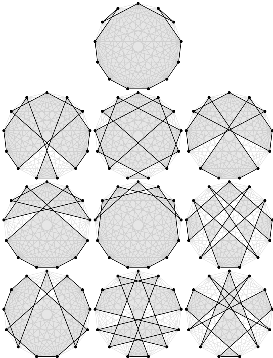
FIGURE 2.9: Replacing the outside path with any of these results in a pre-suitable complex.
