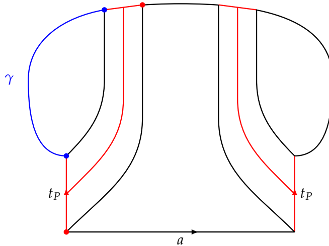
FIGURE 3.56: A disk diagram in \mathcal{P}(S) containing at least two, forced by the three labelled edges, open t_p -corridors.
