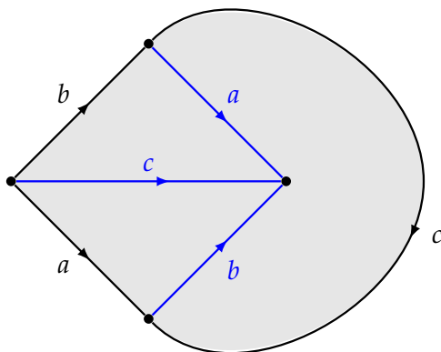
FIGURE 3.26: The resulting standard set of cycles contains cycles reading bac^{-1} , abc^{-1} and cba^{-1} .
