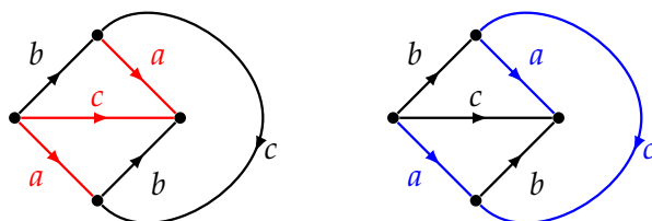
FIGURE 3.30: The two embeddings of ac^{-1}a in \Gamma .
