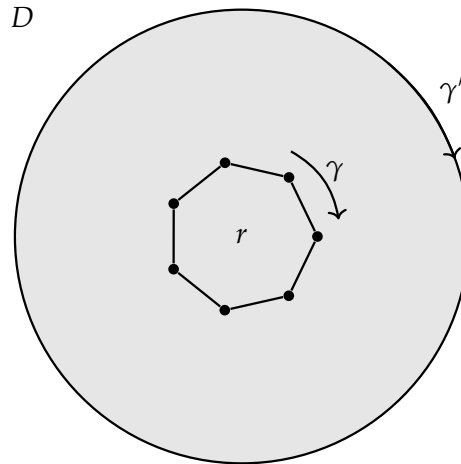
FIGURE 3.46: A van Kampen-reduced disk diagram with boundary length M(\sigma) that contains a relator with boundary word \gamma .
