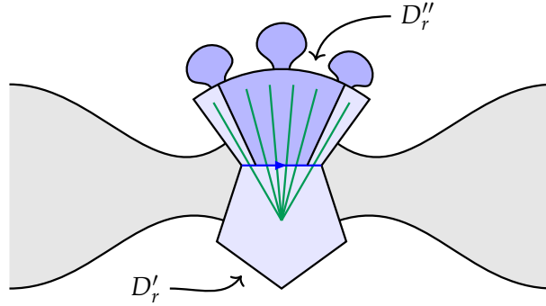
FIGURE 3.19: The entire blue subdiagram is D'_r and the darker subdiagram is D''_r .
