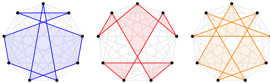
FIGURE 2.7: These polygons define a complex with a significant first homology group.
