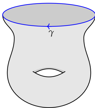
FIGURE 3.47: A surface diagram with boundary \gamma .
