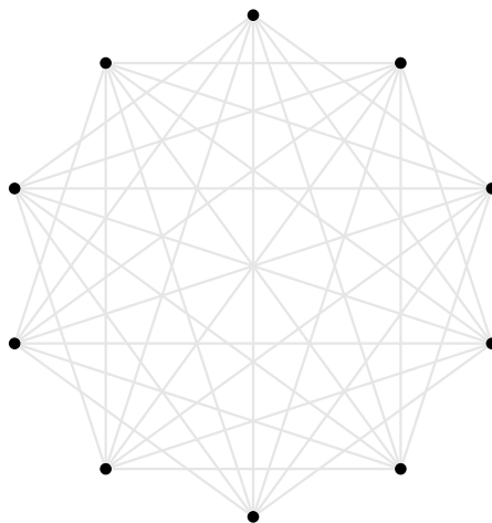
FIGURE 2.16: A graph on 10 vertices with degree 7.
