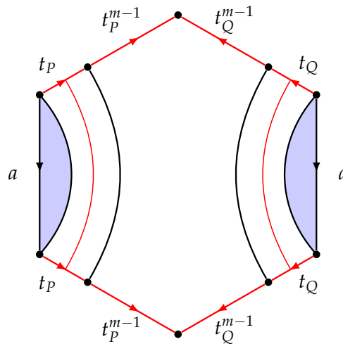
FIGURE 3.54: The boundary of a disk diagram with boundary w .
