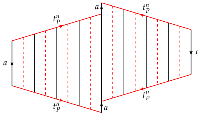
FIGURE 3.50: A van Kampen-reduced disk diagram made up of copies of a single t_P -relator.
