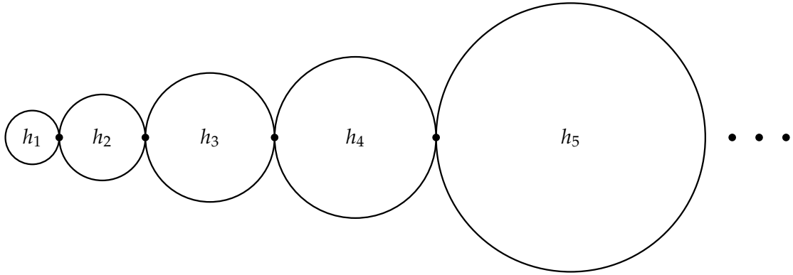
FIGURE 3.45: An infinite graph \Gamma with H(\Gamma) = H .
