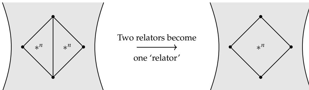
FIGURE 3.8: Two aligned closed path relators are replaced by a single closed path 'relator'. We use quotations as this may not be included in our original set of relators, we will deal with this issue next.
