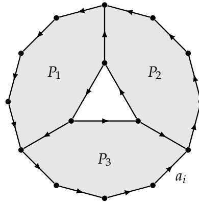
FIGURE 3.1: We assign a direction and label to each edge and label the polygons. For brevity we only present a label for one edge, we assume that all the other edges have their own unique labels.
