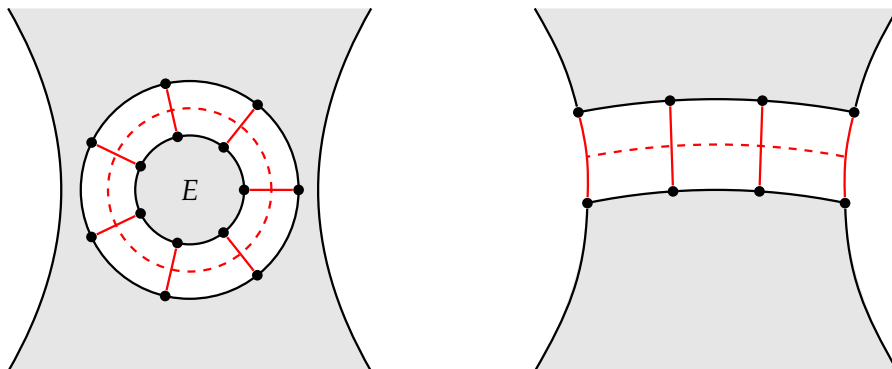
FIGURE 3.12: On the left we have a closed t_P -corridor T where we have used E to label the enclosure (defined below) of T and on the right we have an open t_P -corridor. In each case the red edges represent edges labelled t_P and the dashed line is used to exaggerate the 'corridor-like' behaviour.
