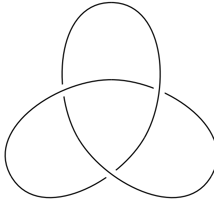
FIGURE 3.41: A representation of the trefoil knot where line breaks represent overlappings.
