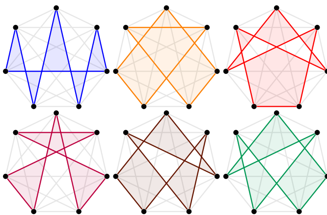
FIGURE 2.6: Each polygon above defines a rotating family that is C'(\frac{1}{6}) with itself and the outside path.
