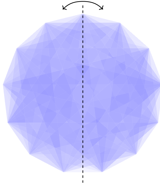
FIGURE 3.52: An automorphism of a suitable complex.
