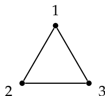
FIGURE 2.10: PGL_2(2) acts 3-transitively on K_3 .
