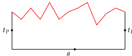
FIGURE 3.55: The edges labelled t_p represent t from Theorem 8.6 and the edge labelled a is our chosen y . The red line represents a potential path from t_p to at_p that does not intersect the path labelled a .
