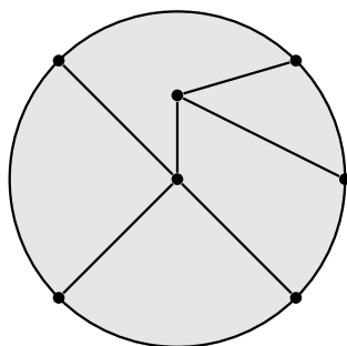
FIGURE 3.44: A graph embedded into a disk.
