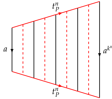
FIGURE 3.49: A van Kampen-reduced disk diagram made up of copies of a single t_P -relator.
