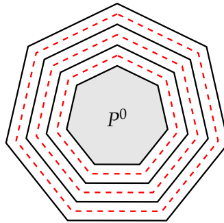
FIGURE 3.48: We realise a surface diagram for P^3 of genus 0.
