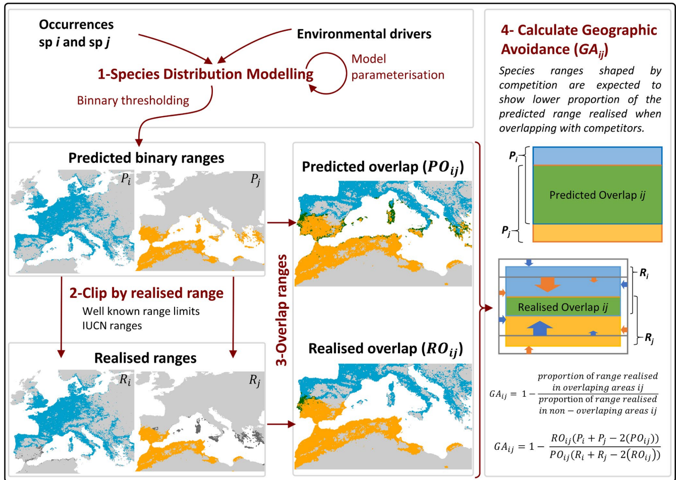
FIGURE 1 Flow chart representing the implementation of the approach to measure geographic patterns of species avoidance expected from macroecological effects of competition. 1—For a given pair of potentially competitor species, occurrence records and species environmental drivers are used to model species' predicted ranges. 2—Binary predicted ranges are cropped by species realised range limits to obtain species' realised ranges. 3—Ranges of both species are combined to estimate extent of overlap in predicted and realised ranges. 4—The measure of Geographic Avoidance ( GA_{ij} ) is applied. In this example, arrows describe a larger decrease from predicted to realised range in areas that overlap with the competitor (large arrows) than in non-overlapping areas (small arrows). Or, equivalently, a lower proportion of realised range occurs in overlapping areas compared to non-overlapping areas. This pattern is described by GA_{ij} with a value > 0
