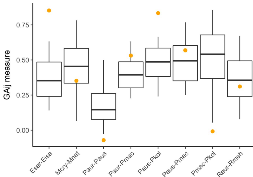
FIGURE 3 Geographic avoidance ( GA_{ij} ) values for each pair of cryptic bat species (orange large dots) relative to null distributions of values (boxplots). Boxes represent first and third data quartiles. Whiskers represent 95 percentiles. (Eser: E. serotinus , Eisa: E. isabellinus . Mesc: M. escaleraei . Mcry: M. crypticus . Paur: P. auritus . Paus: P. austriacus . Pkol: P. kolombatovici . Pmac: P. macrobullaris . Reur: R. euryale . Rmeh: R. mehelyi )
