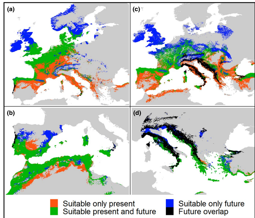
FIGURE 4 Present and future predicted suitable range for E. serotinus (a), E. isabellinus (b), P. austriacus (c) and P. kolombatovici (d) and extent of range overlap with their potential competitors. Orange shows current range that will become unsuitable in future. Green shows current range that will still be suitable in future, and blue shows current unsuitable range that will become suitable. Black shows future suitable range that will overlap with future suitable range of a competitor
