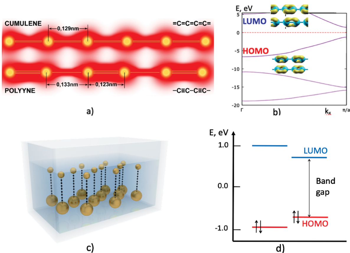
Figure 1. Structure of monatomic carbon chains: (a) Schematic distribution of the electron density in cumulene and polyene allotropes. (b) Band structure of an infinite polyene chain predicted by our ab initio calculation, and the HOMO, LUMO doubly degenerate orbitals. (c) Concept of stabilization of monatomic carbon chains by gold nanoparticles (NPs) in a solution. Gold NPs are shown out of the actual scale. (d) Energy level structure of a finite polyene chain composed by 14 carbon atoms with two gold nanoparticles attached to its ends.
