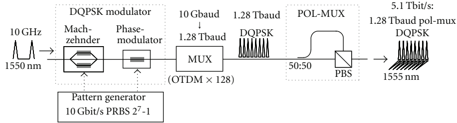
FIGURE 11: 5.1 Tbit/s data generation set-up.
