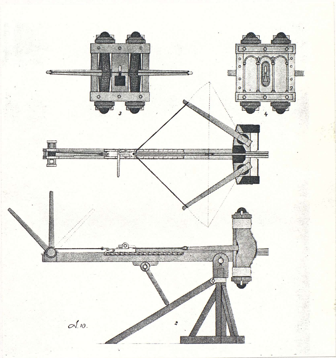
Vitruvian Catapult Capable of firing an arrow 90 cm. in length. (Dr. Baatz, Saalburg Museum)
