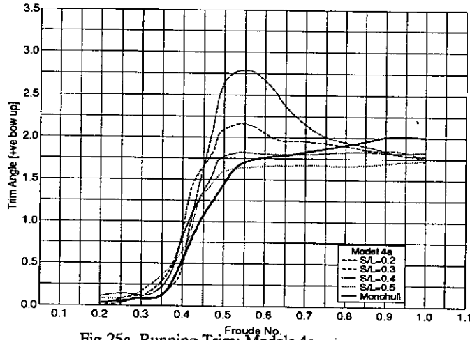
Fig 25a. Running Trim: Models 4a
