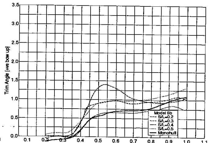
Fig 26c. Running Trim: Models 6b
