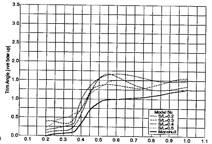
Fig 26b. Running Trim: Models 5b
