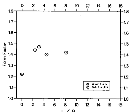
Fig 71b. Form Factors: Model:6b
