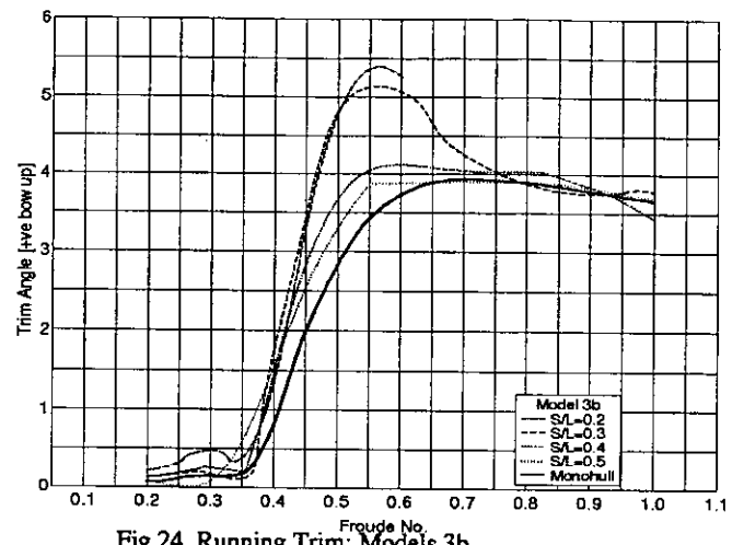
Fig 24. Running Trim: Models 3b
