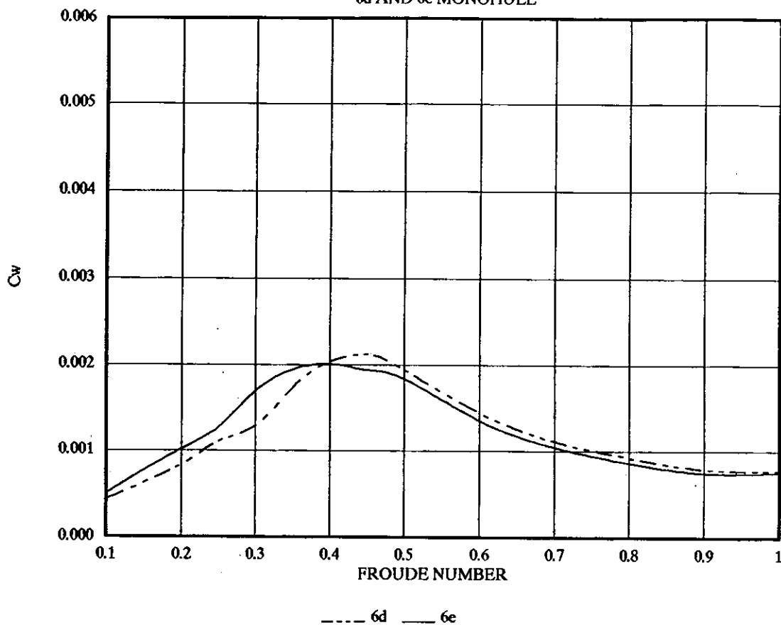
FIGURE 80 THEORETICAL WAVE RESISTANCE C_w (HYDROSTATIC CORRECTION) 6d AND 6e MONOHULL
