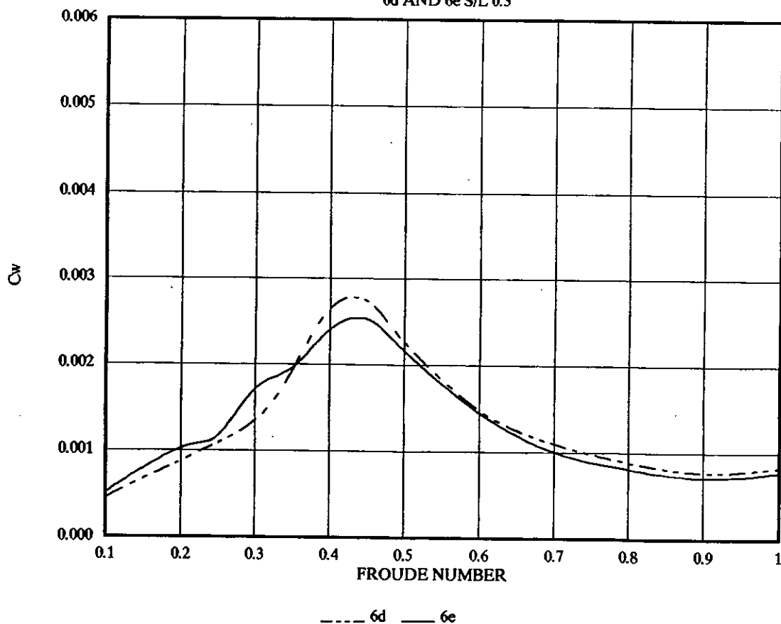
FIGURE 81 THEORETICAL WAVE RESISTANCE C_w (HYDROSTATIC CORRECTION) 6d AND 6e S/L 0.3
