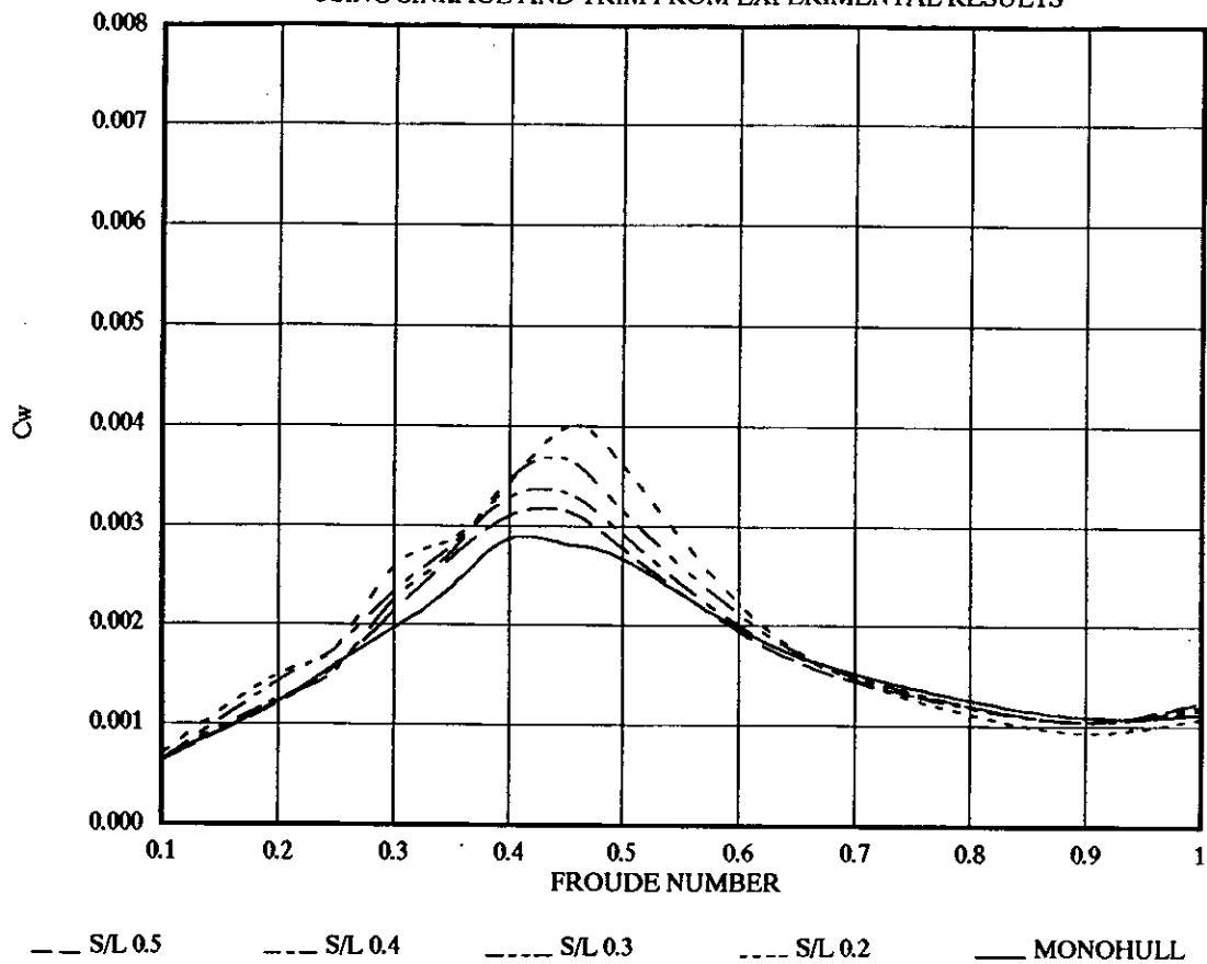
FIGURE 72 THEORETICAL WAVE RESISTANCE FOR 5\epsilon (HYDROSTATIC CORRECTED) USING SINKAGE AND TRIM FROM EXPERIMENTAL RESULTS
