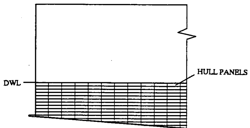
SINGLE SOURCE AT FULL TRANSOM DRAFT AT HALF THE PANEL SPACING
