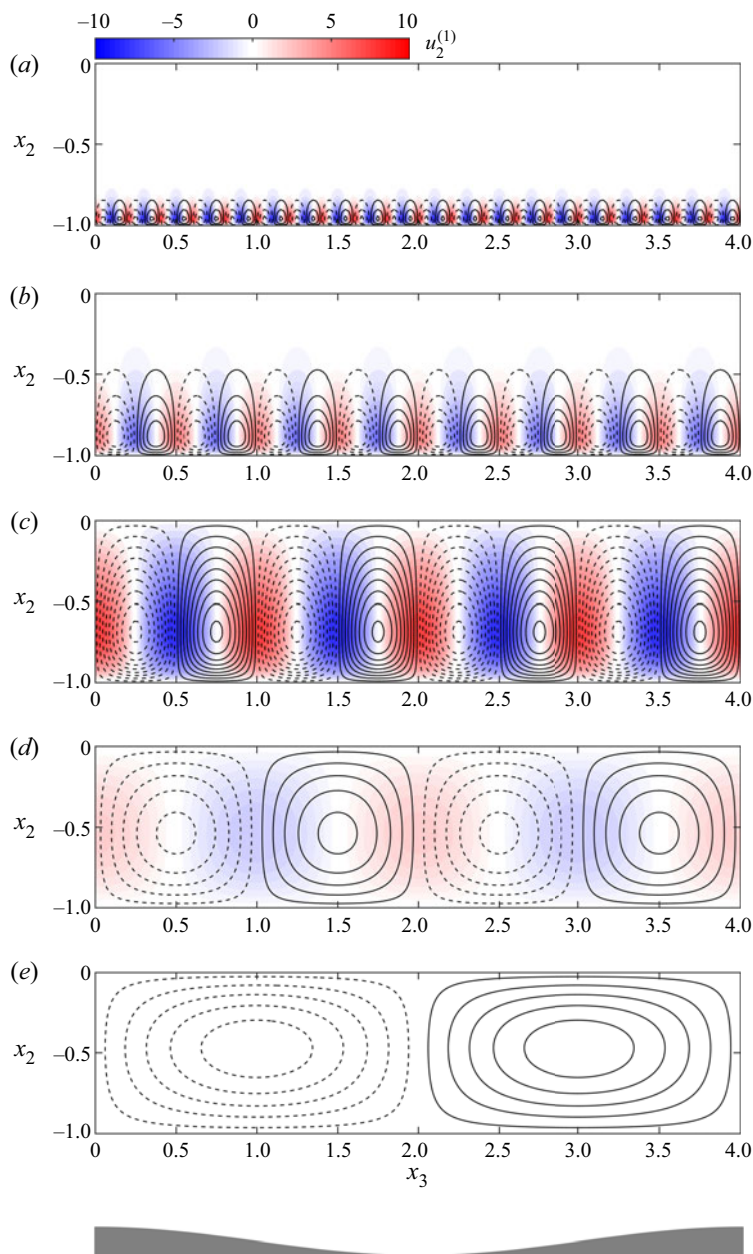
Figure 4. Contours of the perturbation stream function \psi^{(1)} in the cross-plane ( x_2, x_3 ) at Re_\tau = 5200 and varying wavelength: panel (a) \lambda_3 = 0.2 ; panel (b) \lambda_3 = 0.5 ; panel (c) \lambda_3 = 1 ; panel (d) \lambda_3 = 2 ; panel (e) \lambda_3 = 4 . The stream function perturbation is limited to [-1, 1] in panels (a) and (b), to [-2, 2] in panels (c) and (d), to [-0.2, 0.2] in panel (e), for a better representation of the flow structures. Dashed lines are used for negative values. The colour map of the wall-normal velocity perturbation (in units of the friction velocity and per unit of modulation amplitude) is also reported. For wavelengths smaller than \lambda_3 = 4 , the flow topology for a single period is repeated to better display the evolution in size and strength of secondary flows. The topography from crest-to-crest is illustrated for the sake of clarity for \lambda_3 = 4 below panel (e).
