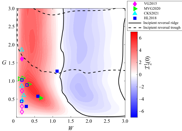
Figure 16. Colour map of the quantity T_2^1(0) as a function of the gap G and width W , for Re_\tau = 5200 . Configurations studied in the recent literature are denoted by symbols (VG2015 for Vanderwel & Ganapathisubramani (2015), MVG2020 for Medjnoun et al. (2020), CKS2021 for Castro et al. (2021) and HL2018 for Hwang & Lee (2018)). Closed symbols denote configurations where downwash over the ridge has been observed. The black lines delimit the regions where the linear model predicts incipient change of flow direction at the midpoint over the ridge (solid line) and at the centre of the trough (dashed line).
