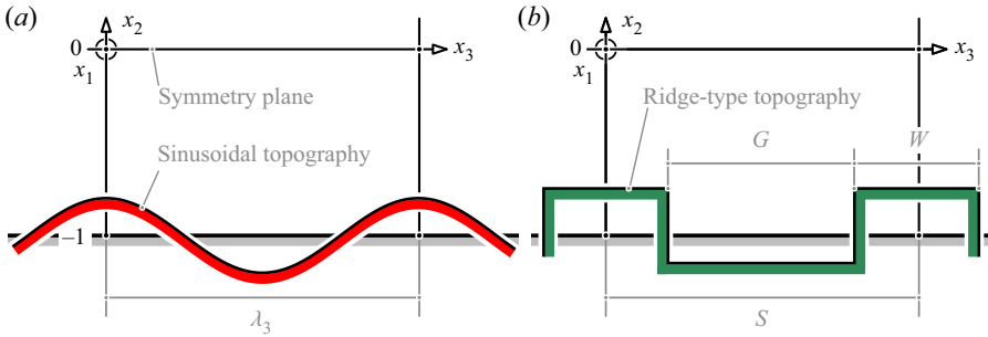
Figure 1. (a) Sinusoidal and (b) ridge-type topographies considered in this paper. The coordinate system (x_1, x_2, x_3) , with origin on the symmetry plane, is shown. The streamwise direction x_1 is oriented into the page. When scaled by h , the mean channel height is equal to 2. Symmetric configurations obtained by mirroring the lower wall geometries shown in the diagrams about the midplane x_2 = 0 are considered. For sinusoidal topographies, the period of the modulation is denoted by \lambda_3 . For ridge-type topographies, the spacing between elements (the period) is denoted by S , while W and G are used to indicate the ridge width and the gap between elements, respectively.
