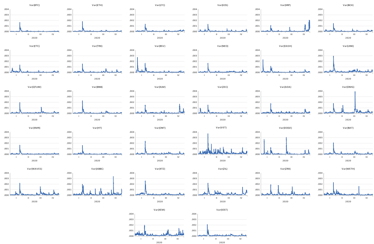
Fig. 6. Diagonal BEKK model conditional variances (COVID-19 period).
