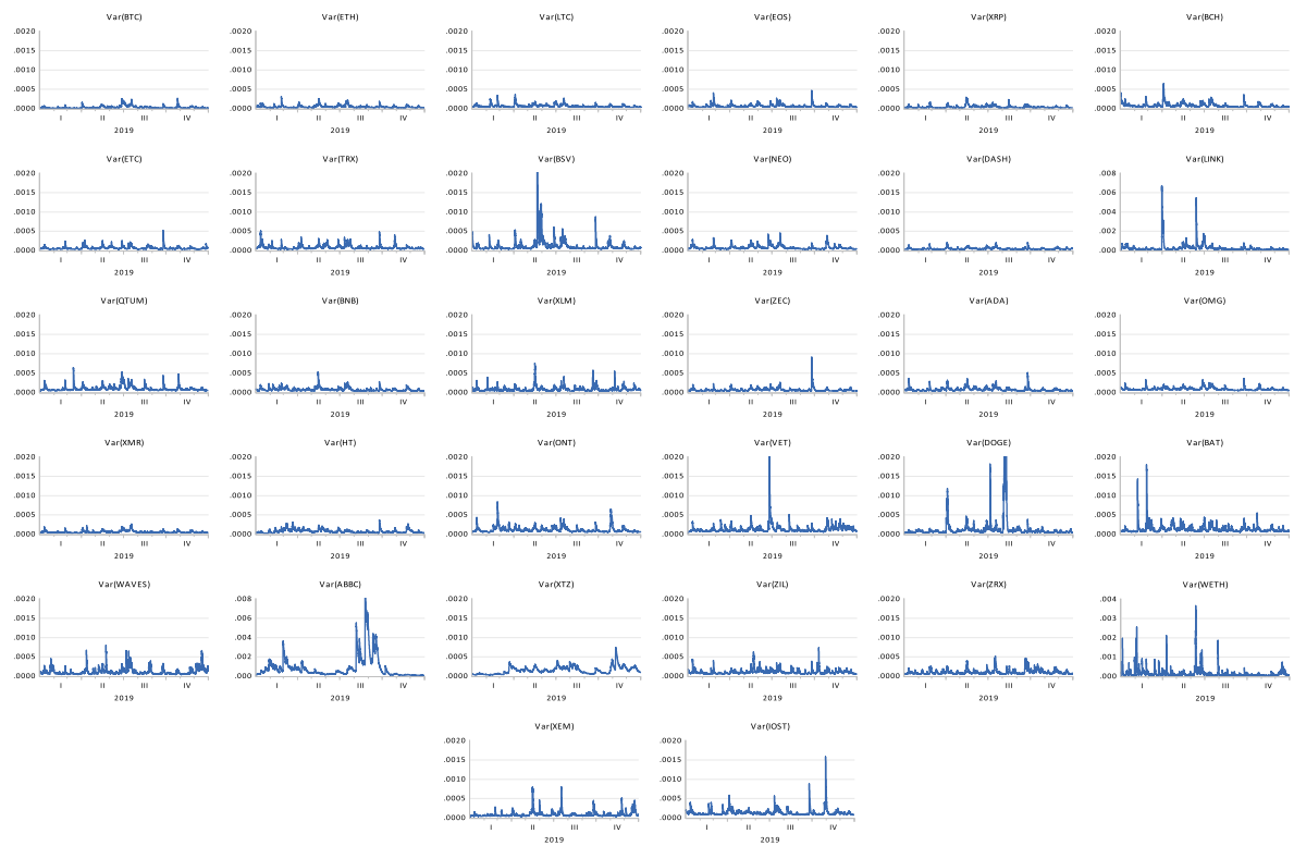
Fig. 5. Diagonal BEKK model conditional variances (pre-COVID period).
