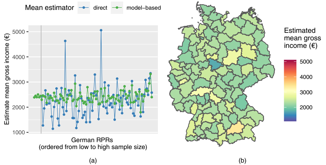
FIGURE 7 (a) The proposed model-based estimates (10) and direct estimates for mean gross individual income per month (€) for German RPRs ordered from low to high sample size and (b) spatial representation of corresponding model-based estimates. The grey line in the left plot separates out-of-sample areas from in-sample areas. For the former only model-based estimates are available. [Colour figure can be viewed at wileyonlinelibrary.com ]
