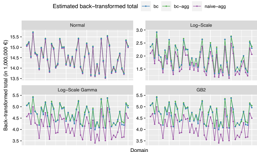
FIGURE 3 Estimated back-transformed totals bc\left(T_i = \sum_{j=1}^{N_i} \exp(\mathbf{x}_{ij}^T \hat{\beta})\right) , bc\text{-}agg\left(\hat{T}_i\right) and naive\text{-}agg\left(\exp\left(\bar{\mathbf{x}}_i^T \hat{\beta}\right)\right) over the domains for one arbitrarily chosen Monte-Carlo simulation. [Colour figure can be viewed at wileyonlinelibrary.com ]
