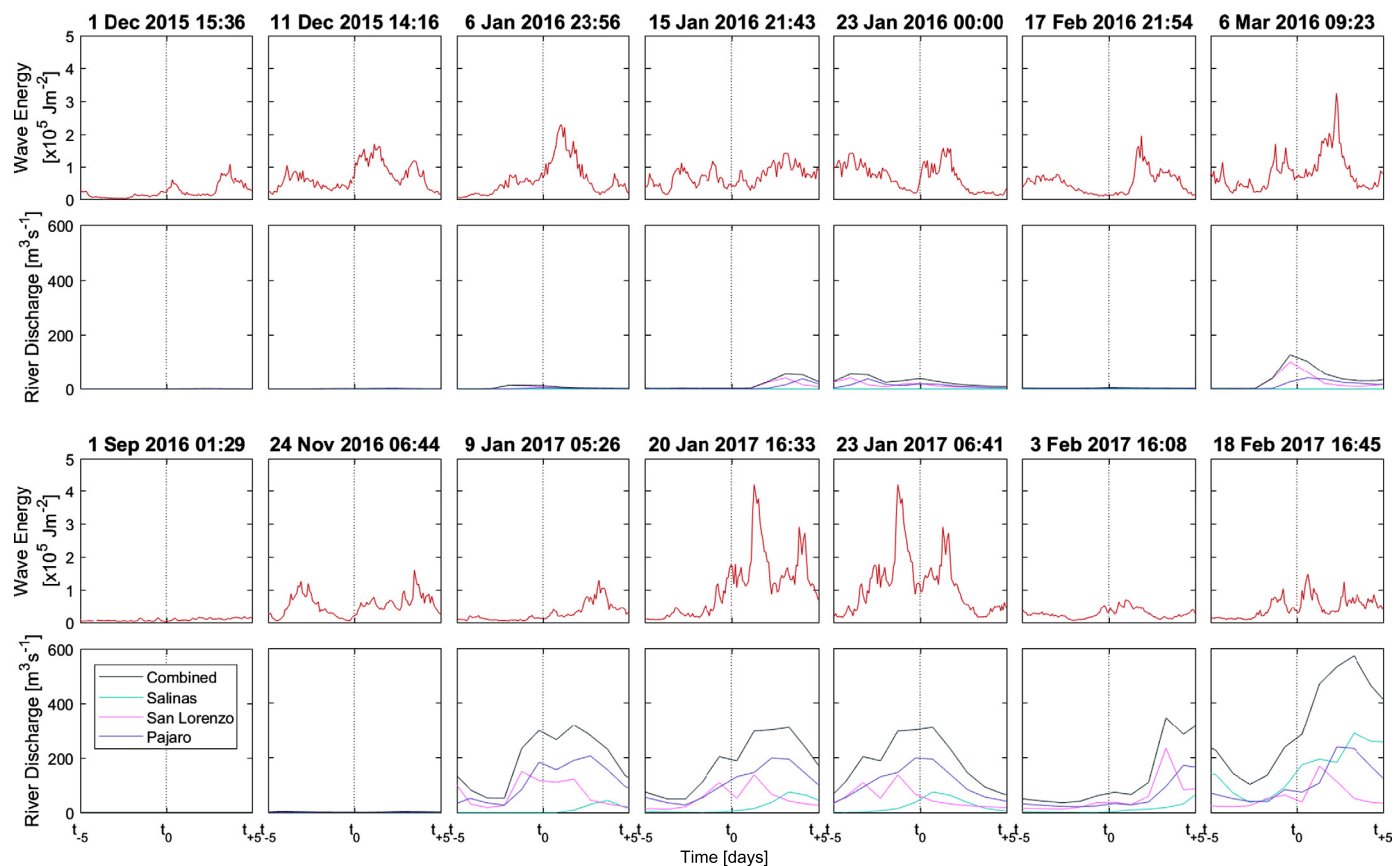
Fig. 4. Measurements of wave energy (red) and San Lorenzo, Pajaro and Salinas Rivers discharge (blue shades), with combined flow (grey) five days prior and following turbidity currents initiating in the upper canyon during the CCE. Central dotted line in each plot indicates the first detection of turbidity current.
