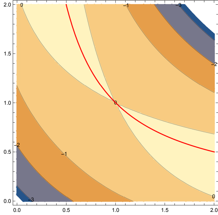
FIG. 4. The entropy given in terms of -g(\varepsilon, \mu) in Eq. (B13) for \varepsilon and \mu between 0 and 2. The contour lines denote the boundaries of regions where the function has values between the designated integers. The positive entropy region is colored lightest (yellow), roughly following the \varepsilon\mu = 1 hyperbola shown in red.
