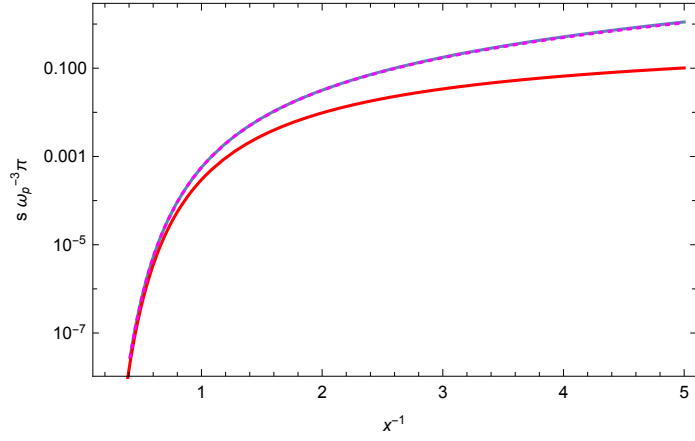
FIG. 3. The exact entropy of the blackbody radiation in the plasma model (upper blue curve) compared with the leading low-temperature asymptotic expression (5.50) (lower red curve) and the numerical integration of the m = 1 term in Eq. (5.47), dotted magenta curve. Even for x = 0.2 , a rather large value of T , the latter is less than 5% low. The cruder approximation (5.50) is only good for rather small values of x^{-1} = 2\pi T/\omega_p .
