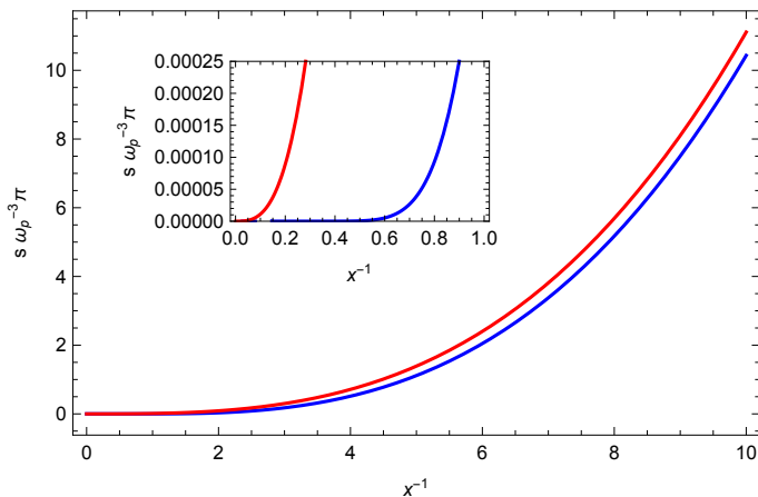
FIG. 2. Comparison of the vacuum entropy density (5.6) (red curve) with the entropy density including plasma-model dispersion, (5.35), (blue curve). These are plotted as functions of x^{-1} = 2\pi T/\omega_p . Both entropy densities tend to zero at zero temperature, and are everywhere positive. The inset shows the behavior for low temperature, and reveals that the plasma-model entropy drops exponentially to zero for relatively large values of the temperature.
