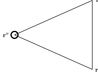
FIG. 1. Sketch of the scattering process used to extract the polarizability of the nanoparticle.
