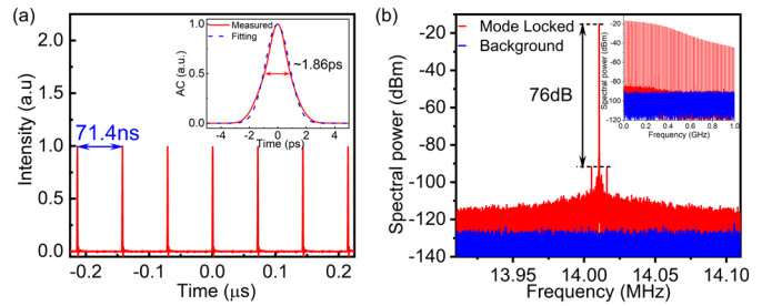
Fig. 3 (a) Oscilloscope trace of the output pulses. Inset: autocorrelation trace of the output pulses. (b) RF spectrum with a RBW of 10Hz and a span of 200kHz at the fundamental frequency of 14.01MHz. Inset: RF spectrum with 1GHz span.
