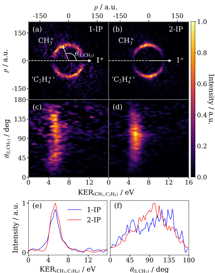
Fig. 7 Newton diagrams for the sequential breakup of (a) 1-IP^{3+} and (b) 2-IP^{3+} into (I^+ + CH_3^+ + C_2H_4^+) in the COM frame of the secondary dissociation C_3H_7^{2+} \rightarrow CH_3^+ + C_2H_4^+ . The Newton diagrams are displayed in polar coordinates in (c) and (d) respectively, where KER_{(CH_3, C_2H_4)} is the KER of the secondary products and \theta_{(I, CH_3)} is the angle between the momenta of the iodine and methyl ions. Each panel is normalised separately. Below are overlaid the integrated KER (e) and angular distributions (f) for both isomers, normalised to unit area.
