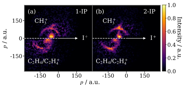
Fig. 5 Newton diagrams for the breakup of (a) 1-IP 2+/3+ and (b) 2-IP 2+/3+ into ( I^+ + CH_3^+ + C_2H_4/C_2H_4^+ ). The correlation of the I^+ and CH_3^+ momenta has been calculated using a contingent covariance analysis. The momentum of the third fragment, assumed to be C_2H_4 or C_2H_4^+ , is deduced through momentum conservation in this frame.
