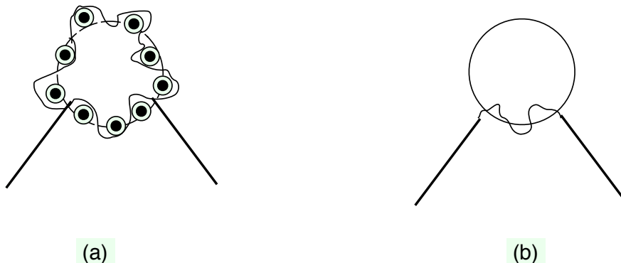
Figure 1: (a) Probing the fuzzball with hard-impact, E \gg T operators causes collective excitations of the fuzzball surface. (b) The corresponding correlators are reproduced in a thermodynamic approximation by the traditional black hole geometry, where we have no fuzzball structure but we use the geometry on both sides of the horizon.
