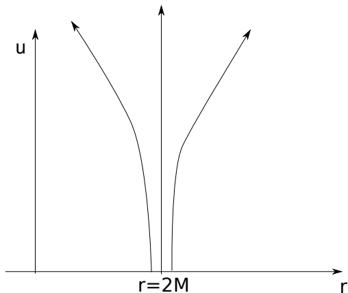
Figure 3: The instability of ‘outgoing geodesics’ at the horizon. The horizontal axis is the radial coordinate, and the vertical axis is an Eddington-Finkelstein coordinate. A null geodesic at r = 2M headed radially outwards stays stuck at r = 2M , one slightly outside escapes to infinity while one slightly inside falls to r = 0 .
