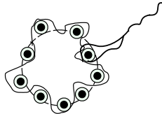
Figure 5: Hawking radiation is just the tail end of the fuzzball structure that ends the geometry outside the horizon; thus there is no natural split between the degrees of freedom on the ‘stretched horizon’ and the degrees of freedom in the Hawking radiation.
