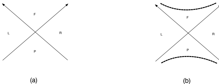
Figure 7: (a) Minkowski space and its Rindler quadrants (Right, Left, Forward and Past). (b) The Penrose diagram of the extended Schwarzschild hole. The region near the intersection of horizons is similar in the two cases.
