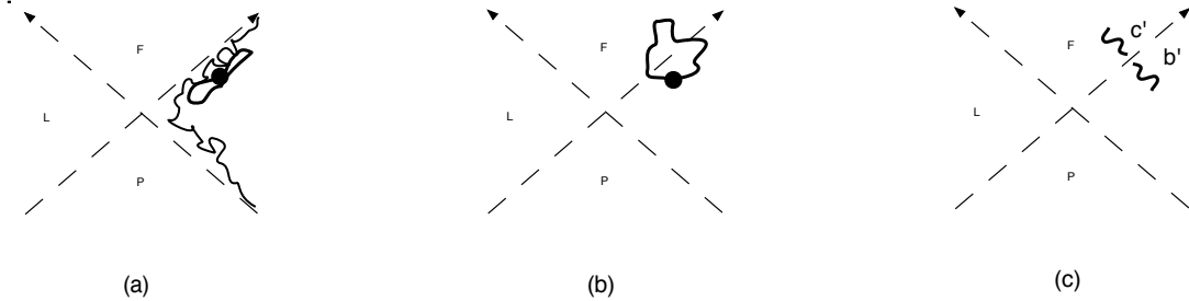
Figure 8: (a) Computing a 1-point function in a generic fuzzball geometry; the operator excites the complicated mess of degrees of freedom on the fuzzball surface (Picture 1). (b) For appropriate operators, the same correlator can be obtained to a good approximation by using the traditional black hole geometry; now there are no degrees of freedom at the horizon but the paths in the path integral can smoothly cross across the horizon into a new auxiliary spacetime region - the black hole interior (Picture 2). (c) In Picture 2, the state is such that we do have modes b', c' entangled as expected in the vacuum.
