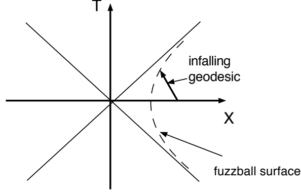
Figure 13: The infalling particle impacting the fuzzball surface.
