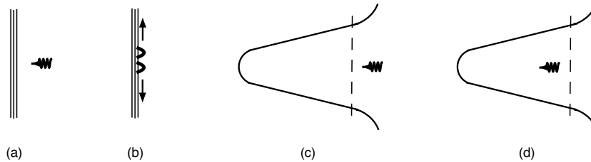
Figure 2: (a) A graviton incident on a stack of D-branes (b) The graviton ‘smashes’ on the branes, converting its energy into a very special state of gluons (collective excitation) (c) The incident graviton in the dual AdS description (d) The graviton passes smoothly through the location where it had appeared to ‘smash’ in the brane description.
