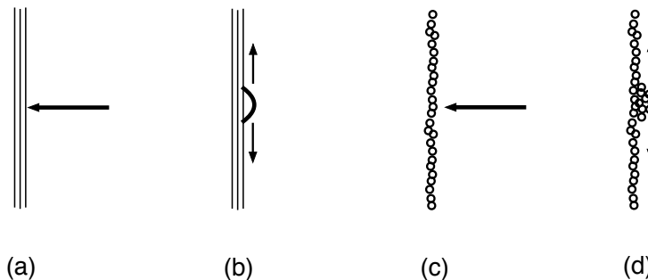
Figure 10: (a) A quantum is incident on a stack of D-branes; (b) The quantum ‘smashes’ on the D-branes, but its energy gets converted into ripples that spread out on the branes; (c) The analogous situation with the fuzzball surface: a graviton is incident on the monopoles etc. making the fuzzball; (d) The graviton ‘smashes’ onto the fuzzball surface, converting its energy to ripples that spread along the fuzzball surface.
