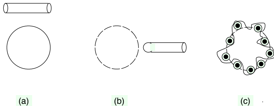
Figure 4: (a) Traditionally, it was assumed that in the black hole geometry the compact directions would appear as a trivial tensor product with the 3+1 metric. (b) In the actual microstates in string theory the compact directions pinch off to make KK monopoles/antimonopoles just outside the place where the horizon would have been. (c) The resulting solutions are ‘fuzzballs’, which have no horizon or ‘interior’.
