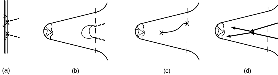
Figure 11: (a) A 2-point function in the CFT: there are some low energy excitations present, but the correlator of interest is not sensitive to them; (b) The dual gravity picture: the low energy excitations are localized deep in the AdS, they do not interfere with the paths contributing to the correlator; (c) One can ask about boundary-bulk propagators in the gravity picture, but these must be re-expressed in terms of boundary-boundary propagators before comparisons can be made with the CFT; (d) A typical process of interaction in the bulk: while this is encoded in the boundary CFT, it is very difficult to extract this encoding from correlators in the CFT.
