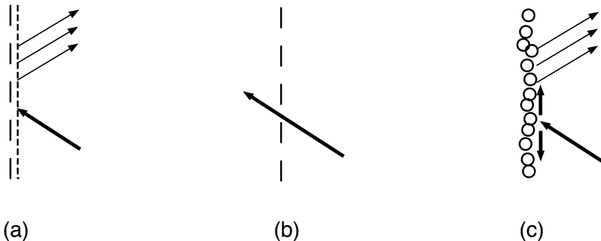
Figure 9: (a) Traditional complementarity: we imagine that infalling matter is absorbed and re-radiated from virtual degrees of freedom at a stretched horizon; these degrees of freedom are virtual because we have found no ‘hair’ for the hole. (b) In the complementary picture, an infalling observer fails to see anything at the location of the stretched horizon. (c) The situation with fuzzballs: real degrees of freedom end the spacetime outside the horizon. These degrees of freedom must play two roles: (i) radiate Hawking quanta at E \sim T and (ii) account for any complementarity through collective oscillations generated by hard impacts of E \gg T quanta.
