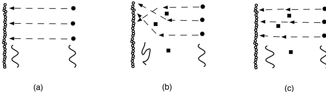
Figure 12: (a) A body made of three atoms (solid dots) falls towards the fuzzball surface. Alternatively, we may consider the wavefunction of a quantum (wavy line). (b) The situation when the interactions with the Hawking radiation quanta are significant: the atoms get scrambled, and the wavefunctions gets severely distorted, all before reaching the fuzzball surface. (c) The situation where the deflections by the Hawking quanta are small; the infalling object retains its character till it reaches the new degrees of freedom available on the fuzzball surface.
