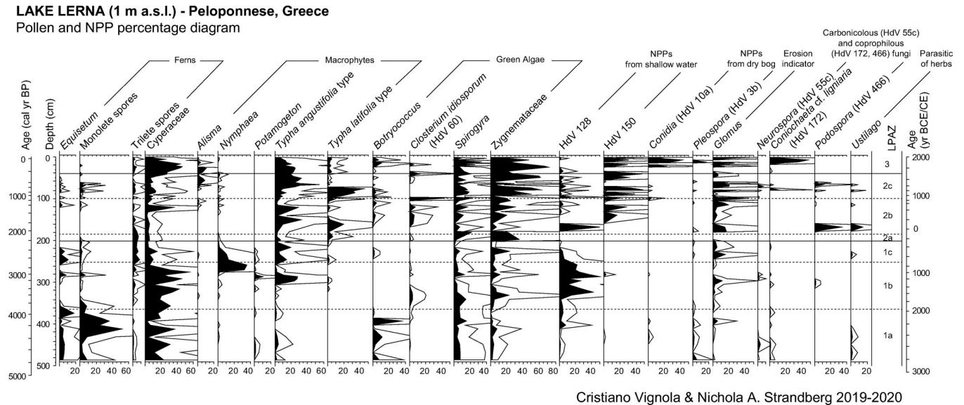
Fig 5. Results of pollen analysis of the study core from ancient Lake Lerna (Peloponnese, Greece). Pollen percentage diagram of selected aquatic and NPP taxa. Curve magnification 4x.
