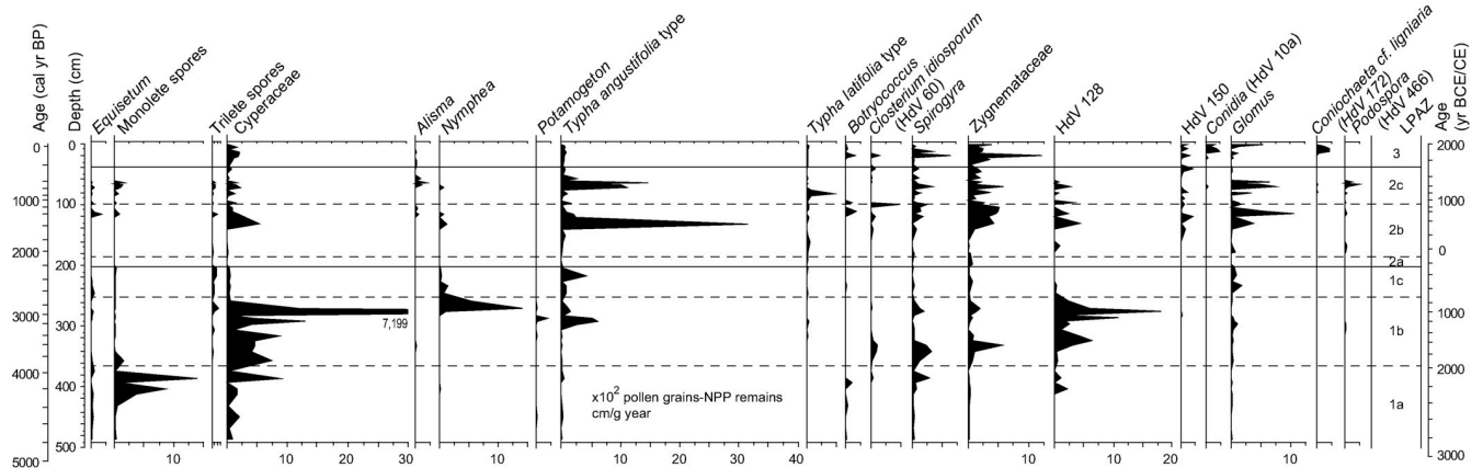
b) Pollen and NPP influx diagram
