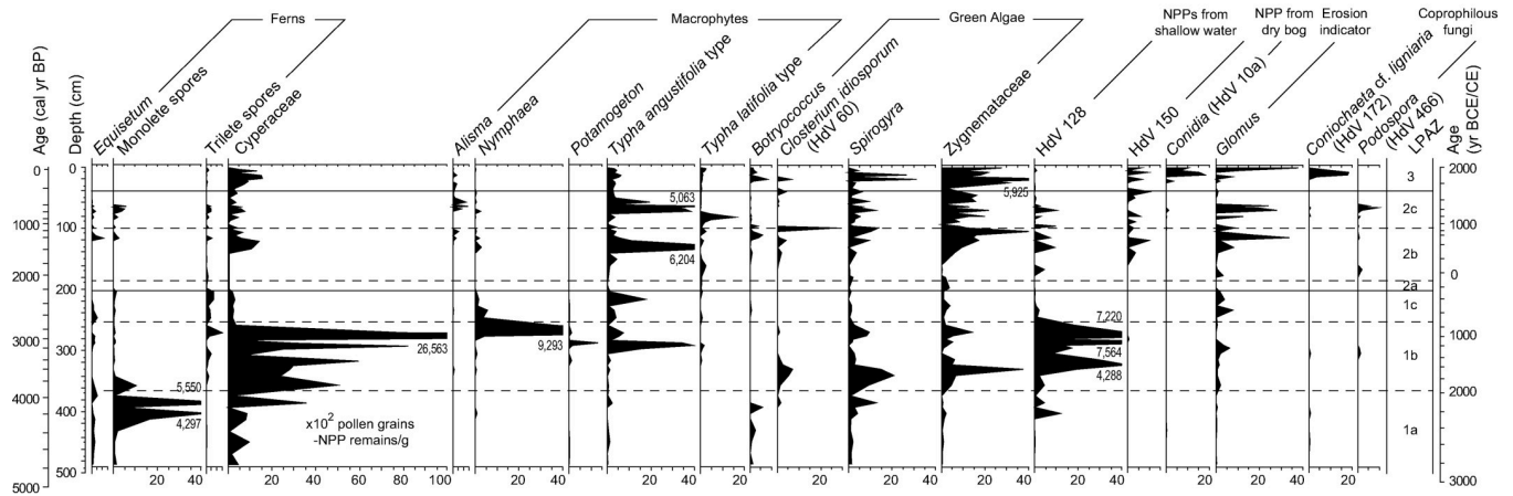
b) Pollen and NPP influx diagram
