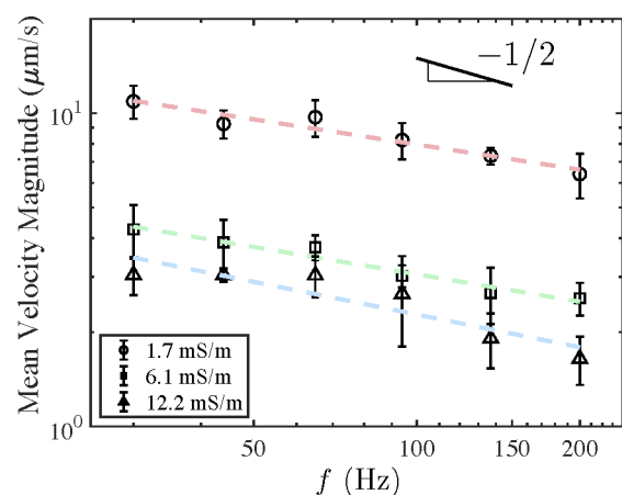
Figure 4. Results of PIV measurements for the average velocity magnitude as a function of frequency of the applied electric field. The amplitude of the applied field was 15 kV/m. Two trends can be clearly observed: the decay of the velocity magnitude with frequency ( f^{-1/2} trend line shown) and with electrolyte conductivity.
