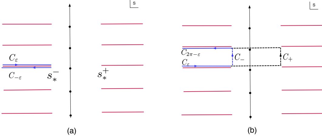
Figure 6. The analytic structure in the complex s -plane. The original integral is over the solid blue lines. On the future horizon, we complete the contour by including the dashed blue lines. On the past horizon, we complete it by including the dashed grey line at s_*^- .
