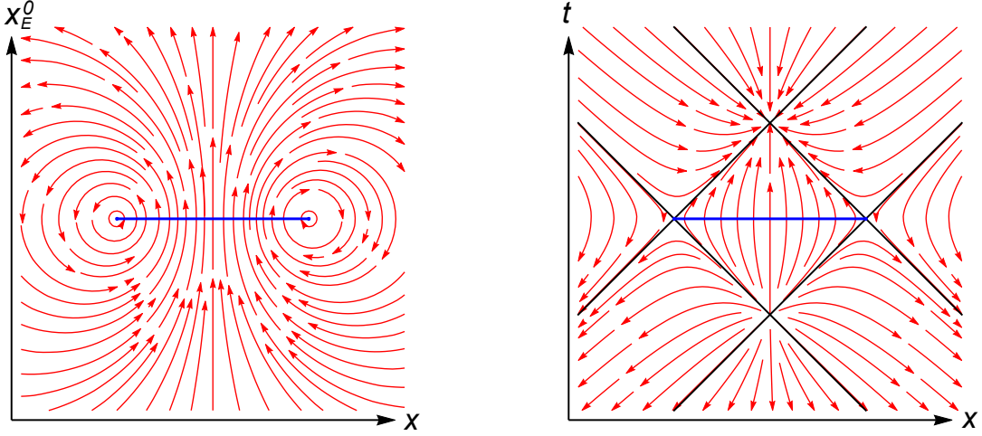
Figure 2. The flow generated by the modular Hamiltonian of the region A (in blue). We start by working in Euclidean time x_E^0 , depicting the vector field \partial_\tau on the left. The calculation then introduces an imaginary shift in \tau , which results in a displacement of the operator insertion into real time t . The picture of the real time vector field \partial_s = \frac{1}{2\pi}\zeta_A is shown on the right with the causal structure indicated in gray. The two plotted planes can be thought of as orthogonal to each other and sewn together along the region A .
