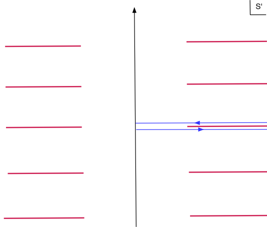
Figure 8. The analytic structure in the complex s' = s_B - s plane. The red lines are branch-cuts. The blue line is the contour of integration.
