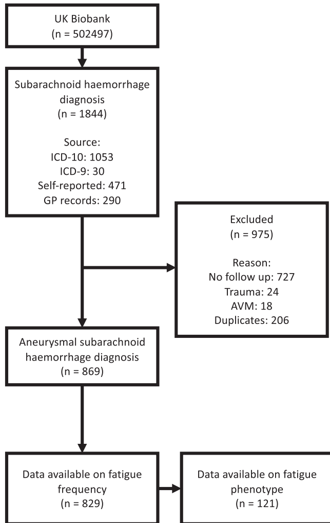
FIGURE 1 aSAH sample inclusion flowchart for UK Biobank
