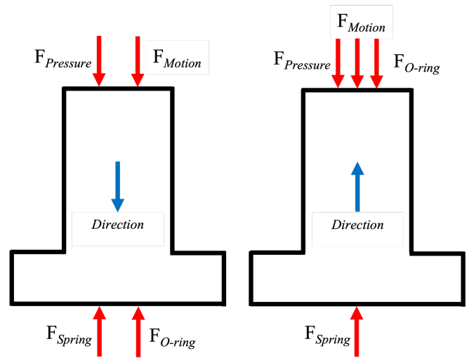
Fig. 4. Free body force diagram for contraction (left) and expansion (right) of the piston
