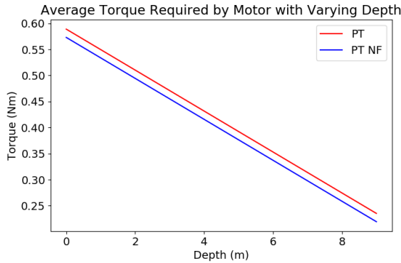
Fig. 5. Average Motor Torque required as depth varies
