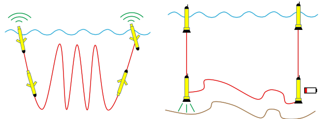
Fig. 1. Illustration of contrasting submersible dive profiles, showing typical glider (left) and typical Lagrangian imaging float (right) missions
