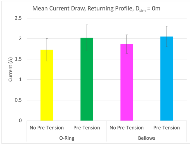
Fig. 13. Mean current draw during RP tests for all configurations, D_{Sim} = 0
