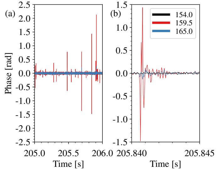
Fig. 4. Greater detail of single events between 205 and 206 s; same data as in Figure 3 without any downconversion. (a) 1 second of DAS data, distances: 154m before pressboard in black, 159.5m within pressboard in red, 165m after pressboard in blue. (b) Greater detail across time frame of 5 ms showing an impulse-like single PD event in DAS data at pressboard location.
