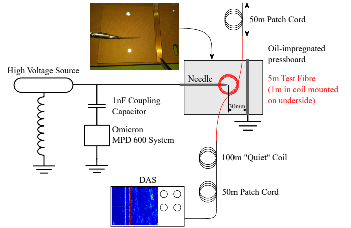
Fig. 2. Mixed electrical and optical schematic of the pressboard setup comprising of the DAS firing through the patch and quiet coils into the 5 m of test section of which 1 m is mounted to the pressboard; as well as electrical omicron measurement connected in parallel with the HV source. Needle is set at 30mm from the grounded bar at an angle of 10^\circ .
