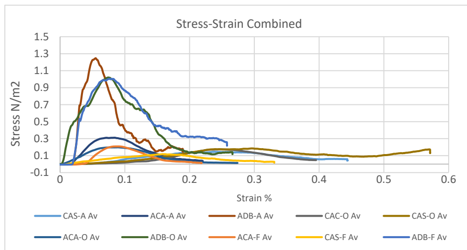
Figure 3 Stress-Strain graph
