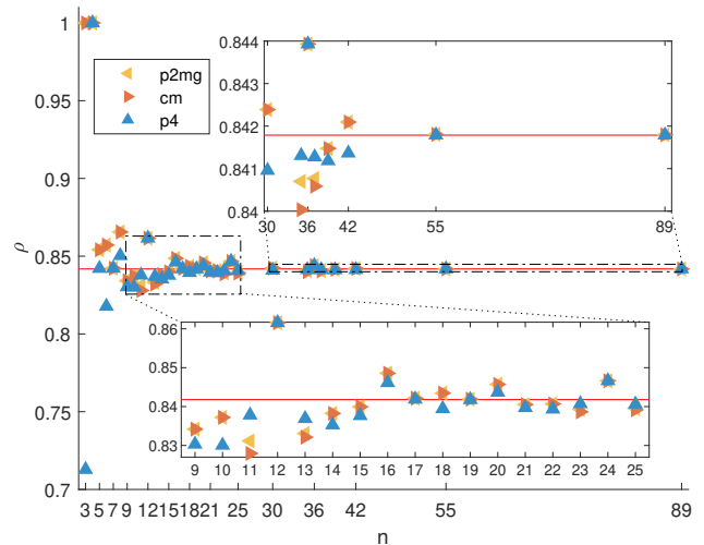
FIG. 4: Densities of the densest packings of examined n -gons in the p2mg/cm/p4 plane groups class. The red line denotes the density of the in this plane group class.
