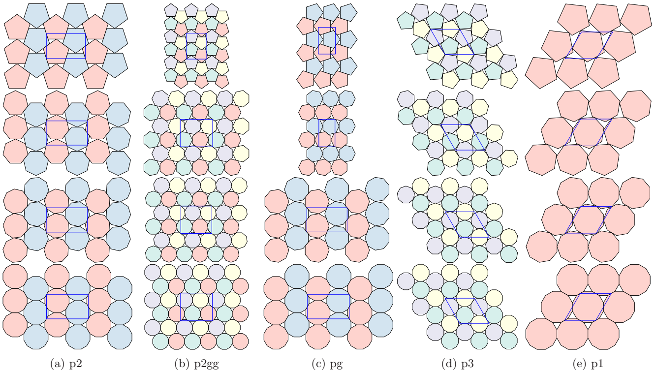
FIG. 2: Densest configurations of (from top to bottom) pentagon, heptagon, enneagon and dodecagon in plane groups p2 , p2gg , pg , p3 , and p1 with the following densities: pentagon in p2/p2gg/pg \approx 0.92131 , p3 \approx 0.87048 and p1 \approx 0.81725 ; heptagon in p2/p2gg/pg \approx 0.89269 , p3 \approx 0.88085 and p1 \approx 0.86019 ; enneagon in p2 \approx 0.90103 , p2gg \approx 0.89989 , pg \approx 0.89860 and p3/p1 \approx 0.88773 ; dodecagon in p2/p2gg/pg/p3/p1 \approx 0.92820 . The blue parallelogram denotes the primitive cell of the respective configuration. Colors represent symmetry operations modulo lattice translations.
