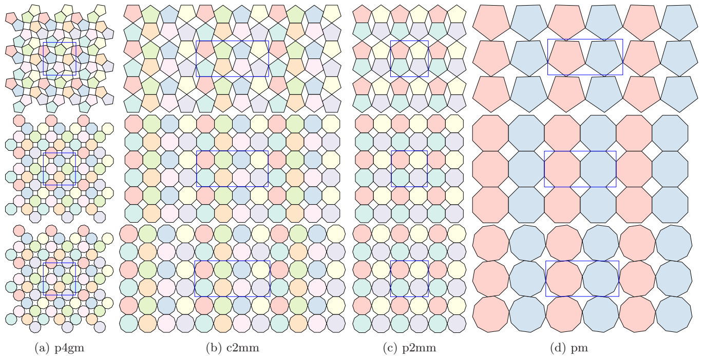
FIG. 7: Densest configurations of (top) pentagon, (middle) octagon and (bottom) decagon in plane groups p4gm , c2mm , p2mm and pm with the following densities: pentagon in p4gm \approx 0.71119 , c2mm \approx 0.71714 and p2mm/pm \approx 0.69098 ; octagon in p4gm/c2mm/p2mm/pm \approx 0.82842 ; decagon in p4gm \approx 0.77205 and c2mm/p2mm/pm \approx 0.77254 . The blue parallelogram denotes the primitive cell of the respective configuration. Colors represent symmetry operations modulo lattice translations.
