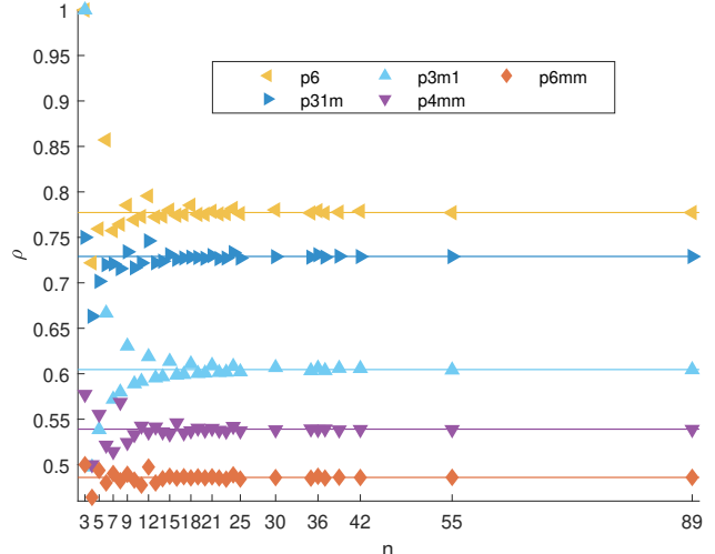
FIG. 10: Densities of the densest packings of examined n -gons in the p6/p31m/p3m1/p4mm/p6mm plane groups class. The coloured lines denote the density of the corresponding densest plane group disc packings.
