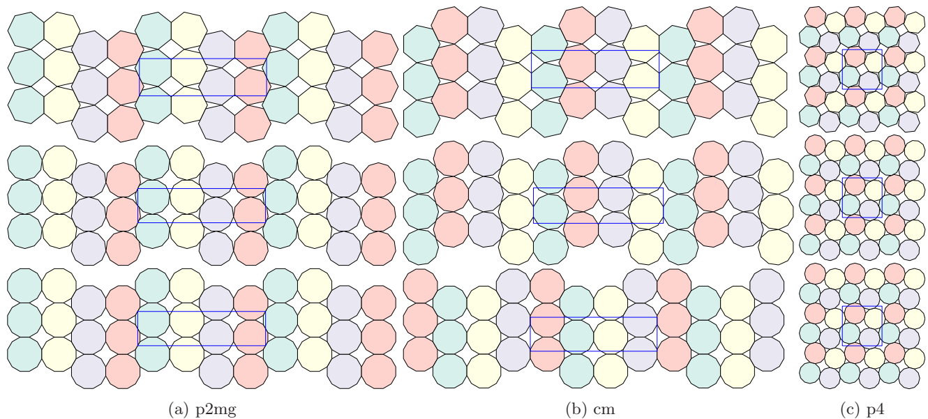
FIG. 5: Densest configurations of (top) heptagon, (middle) endecagon and (bottom) dodecagon in plane groups p2mg , cm , and p4 with the following densities: heptagon in p2mg/cm \approx 0.84226 and p4 \approx 0.84219 ; endecagon in p2mg \approx 0.83116 , cm \approx 0.82795 and p4 \approx 0.83780 ; dodecagon in p2mg/cm/p4 \approx 0.86156 . The blue parallelogram denotes the primitive cell of the respective configuration. Colors represent symmetry operations modulo lattice translations.
