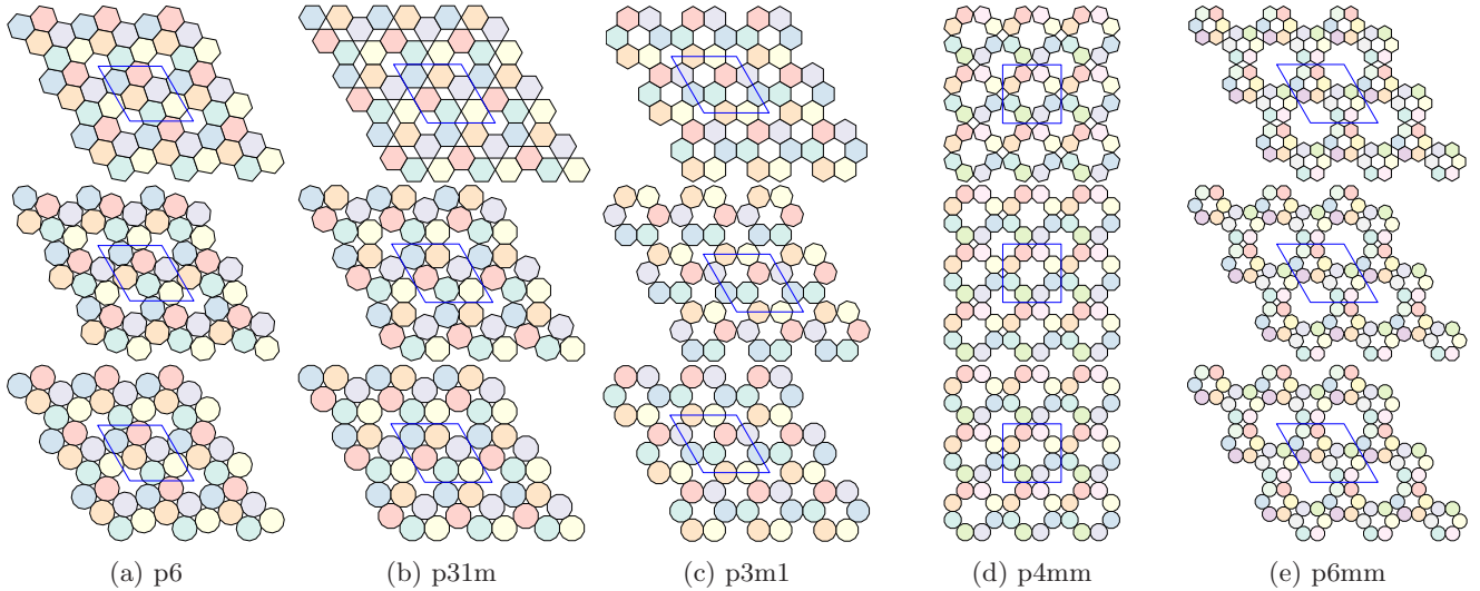
FIG. 11: Densest configurations of (from top to bottom) hexagon, octagon and dodecagon in plane groups p6 , p31m , p3m1 , p4mm , and p6mm with the following densities: hexagon in p6 \approx 0.85714 , p31m \approx 0.71999 , p3m1 \approx 0.66666 , p4mm \approx 0.52148 and p6mm \approx 0.47999 ; octagon in p6 \approx 0.76438 , p31m \approx 0.71565 , p3m1 \approx 0.57980 , p4mm \approx 0.56854 and p6mm \approx 0.48235 ; dodecagon in p6 \approx 0.79560 , p31m \approx 0.74613 , p3m1 \approx 0.61880 , p4mm \approx 0.53589 and p6mm \approx 0.49742 . The blue parallelogram denotes the primitive cell of the respective configuration. Colors represent symmetry operations modulo lattice translations.
