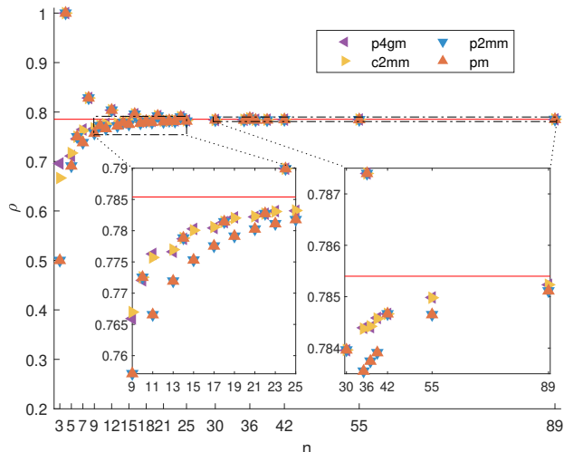
FIG. 9: Densities of the densest packings of examined n -gons in the p4gm/c2mm/p2mm/pm plane groups class. The red line denotes the density of the densest disc packing in this plane group class.
