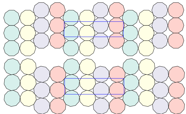
FIG. 6: Two non-isomorphic densest p2mg packings of a decagon obtained by ETRPA with packing density of approximately 0.83722.
