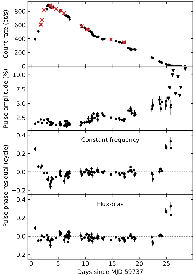
Figure 1. Outburst evolution of MAXI J1816 relative to 2022 June 7 (MJD 59737). The top panel shows the 0.5 – 10 keV count-rate as a function of time, with each point representing a single NICER pointing. The X-ray bursts have been removed from this data, but their onset times are marked with red crosses. The second panel shows the fractional pulse amplitude in the 0.5 – 10 keV range using triangles to indicate 95% upper limits for non-detections. Finally, the two bottom panels give the phase residuals relative to a constant frequency and flux-bias adjusted timing model (see Table 1).
