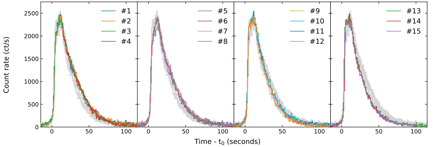
Figure 2. Light curves of the 15 X-ray bursts observed from MAXI J1816. These light curves are calculated in the 0.5 – 10 keV energy range at 1 s resolution, with the preburst count-rate subtracted. In each panel a different subset of the bursts are highlighted in color (with the burst number as in Table 2), while the remaining bursts are shown in gray for comparison.
