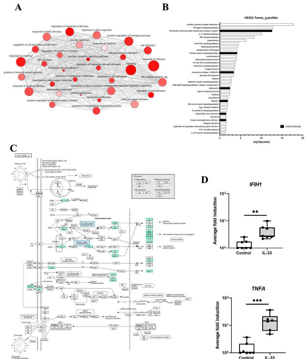
Figure 2. IL-33 induced DEGs associated with viral immunity in MCs. (A), gene enrichment map of GO terms analysed using g.profiler. (B), top KEGG pathways 6 h post IL-33 (10 ng/mL) treatment, n = 7 . (C), genes associated with the influenza Pathway using KEGG on DEGs 6 h post IL-33 (10 ng/mL) treatment, n = 7 . (D), mRNA expression of genes ( IFIH1 , TNFA ) in influenza pathway 6 h post IL-33 stimulation (10 ng/mL), n = 7 . ** p \leq 0.01 , *** p \leq 0.001 for control versus IL-33.
