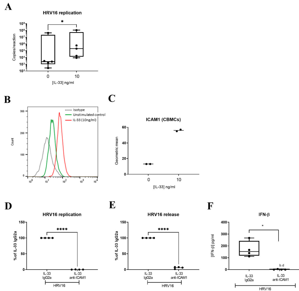
Figure 6. Role of ICAM1 in mediating IL-33-dependent enhancement of HRV16 replication in CBMCs. Viral RNA in CBMCs pretreated with or without IL-33 (10 ng/mL) for 24 h prior to HRV16 infection (MOI 7.5) for a further 24 h, n = 5 (A). A representative flow cytometric trace (B) and averaged geometric mean (C) for ICAM1 cell surface expression in MCs treated with IL-33 (10 ng/mL) for 24 h, n = 2 . HRV16 replication (D), virion release (E) and IFN- \beta release (F) following IL-33 (10 ng/mL) stimulation for 24 h prior to HRV16 infection (MOI 7.5) in the presence or absence of anti-ICAM1 antibody or IgG2a isotype for a further 24 h, n = 4 . * p \leq 0.05 for no cytokine versus IL-33 and * p \leq 0.05 , **** p \leq 0.0001 for IL-33 IgG2a+HRV16 versus IL-33 anti-ICAM1+HRV16.
