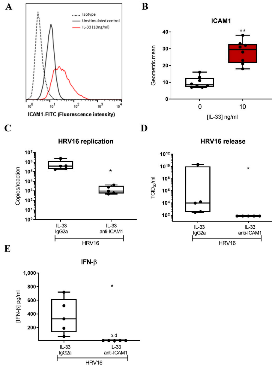
Figure 5. Role of ICAM1 in mediating IL-33-dependent enhancement of HRV16 replication in LAD2 MCs. A representative flow cytometric trace (A) and averaged geometric mean (B) for ICAM1 cell surface expression in MCs treated with IL-33 (10 ng/mL) for 24 h, n = 8 . HRV16 replication (C) and virion release (D) and IFN- \beta protein release (E) following IL-33 (10 ng/mL) stimulation for 24 h prior to HRV16 infection (MOI 7.5) in the presence or absence of anti-ICAM1 antibody or IgG2a isotype for a further 24 h, n = 5 . ** p \leq 0.01 for no cytokine versus IL-33 and * p \leq 0.05 for IL-33 IgG2a+HRV16 versus IL-33 anti-ICAM1+HRV16.
