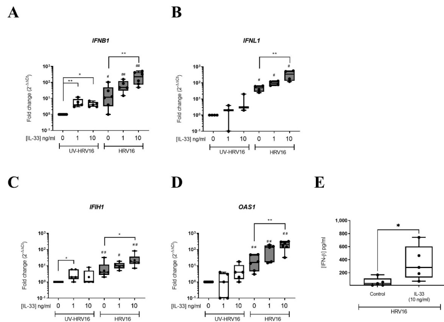
Figure 3. IL-33 enhanced HRV16-dependent anti-viral responses in MCs. mRNA expression of IFNs IFNB1 (A), IFNL1 (B) and IFN-stimulated genes IFIH1 (C), OAS1 (D) and IFN- \beta protein (E) in LAD2 MCs pretreated with or without IL-33 (1–10 ng/mL) for 24 h prior to HRV16 or UV-HRV16 (control) infection (MOI 7.5) for a further 24 h, n = 3–6 . * p \leq 0.05 , ** p \leq 0.01 for no cytokine versus IL-33 (1 or 10 ng/mL). # p \leq 0.05 , ## p \leq 0.05 for UV-HRV16 versus HRV16.
