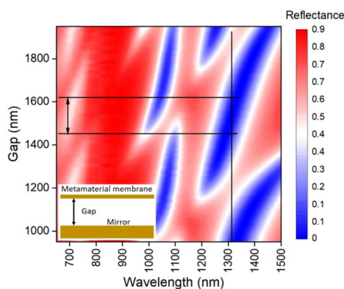
Fig. 6 Dependence of metamaterial-microcavity reflectance on gap and wavelength according to the inverse design parameters of the metamaterial. Inset is the 2D illustration of the metamaterial-microcavity.
