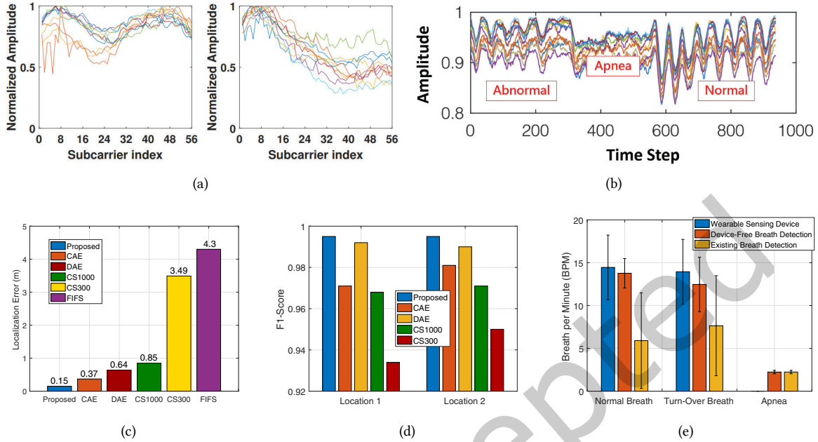
Fig. 9. Experimental results of (a) CSI for presence observations and (b) CSI for abnormal/normal/apnea breathing scenarios and the corresponding performances of (c) localization [223], (d) presence detection [97] and (e) breath rate detection in terms of localization errors, F1-score and rate of breath per minute (BPM), respectively.
