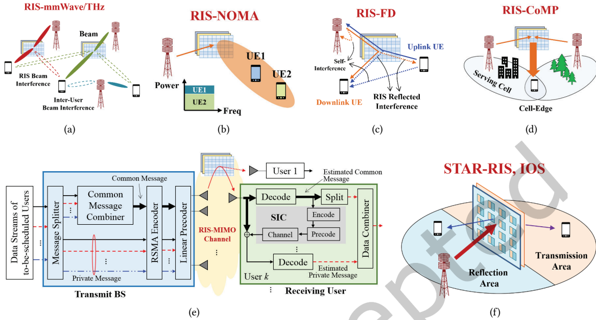
Fig. 3. The 6G RIS-empowered wireless network of (a) RIS-empowered mmWave/THz (b) RIS-NOMA (c) RIS-FD and (d) RIS-CoMP transmissions as well as emerging architecture of (e) RSMA and (f) STAR-RIS/IOS.
