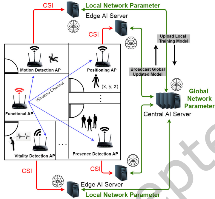
Fig. 8. Device-free wireless positioning and sensing detection with the deployed functional APs, edge and central AI servers. The CSI dataset is collected via wireless channels between AP pairs. Local network parameters are learned by edge AI servers, whereas global model updating and broadcasting are performed by a central AI server.
