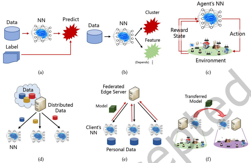
Fig. 10. Deep learning mechanisms of (a) supervised, (b) unsupervised, and (c) reinforcement learning. The architecture of network learning of (d) distributed, (e) federated and (f) transfer learning.
