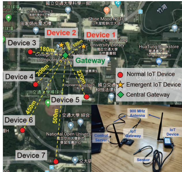
Fig. 7. Experimental environment of an LoRa-based IoT network [204].
