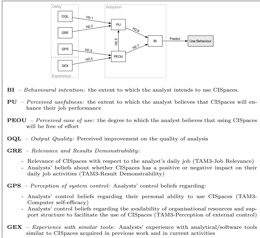
Figure 11: Technology Acceptance Model TAM-A adapted for the study
