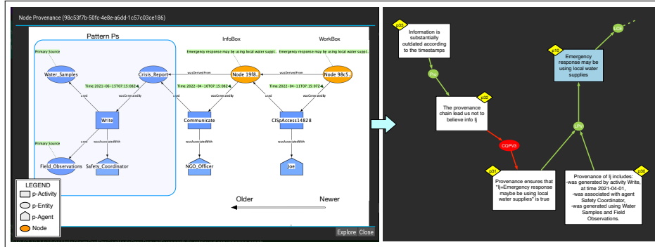
Figure 9: Provenance chain associated to p_{10} : “Emergency response may be using local water supplies,” cf. Fig. 5, and conflict that can be generated.
