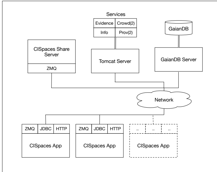
Figure 10: CISpaces system architecture
