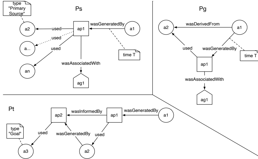
Figure C.19: Patterns used to query a provenance chain of nodes p_i in CISpaces
