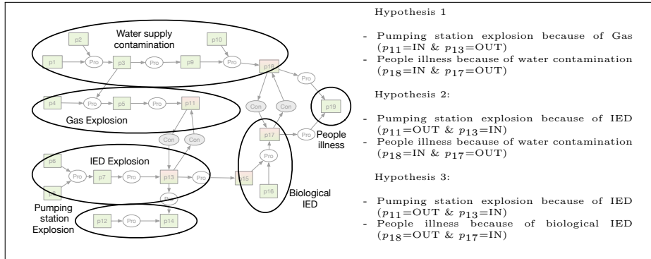
Figure 7: CISpaces analysis and evaluation: Three alternative hypotheses.
