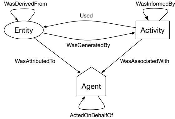
Figure C.18: The PROV-DM core [55]
