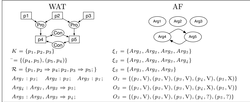
Figure A.14: WorkBox Argumentation Theory (WAT) and its translation first into ASPIC, and then into a Dung’s Argumentation Framework to derive preferred extensions and hence intelligence analysis hypotheses.
