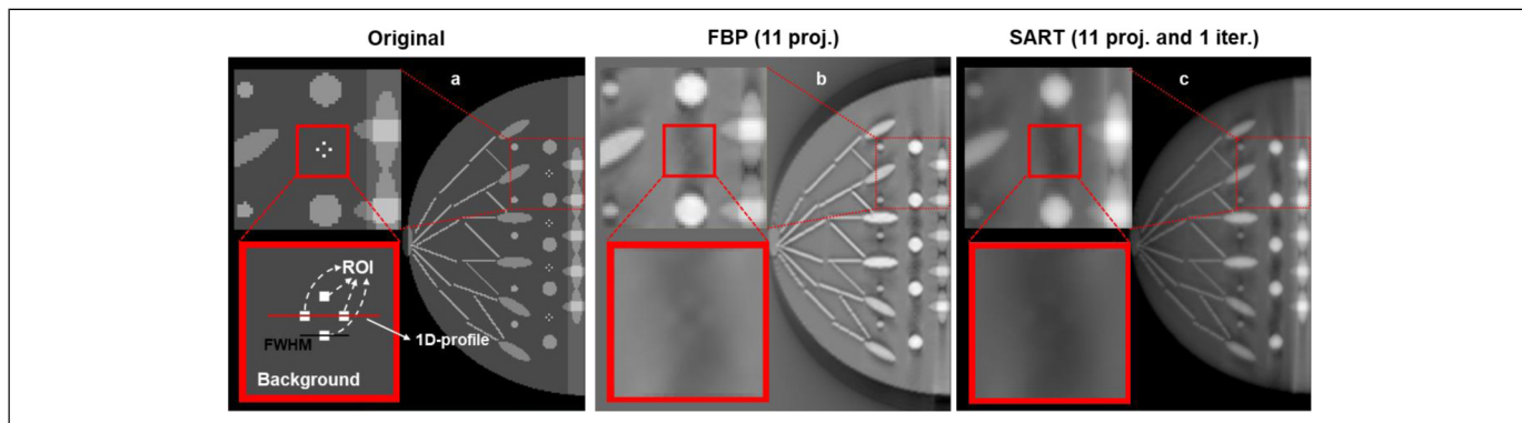
Figure 3. The comparison of the original layer of interest (LOI) (128th slice) (a), the reconstructions of LOI via filtered back projection (FBP) (b), and simultaneous algebraic reconstruction technique (SART) (1 iteration) (c) for 11 projections. (a) The description of region of interest (ROI), background of ROI, full width half maximum (FWHM) line, and 1D profile line.
