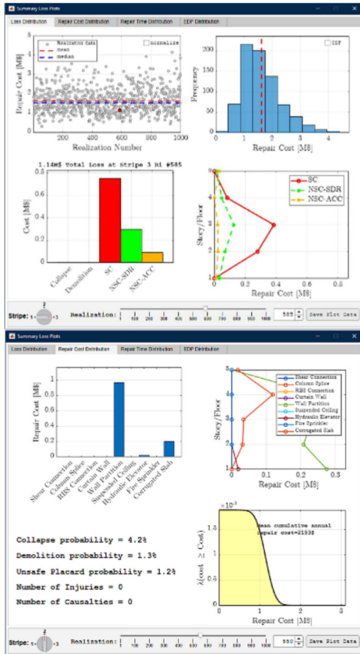
Figure 10. Summary plot interface for the FEMA P-58 option.
