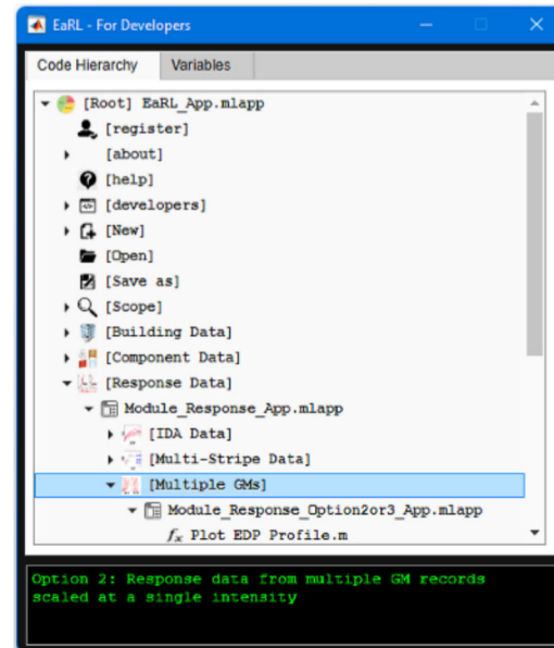
Figure 11. Developers interface.
