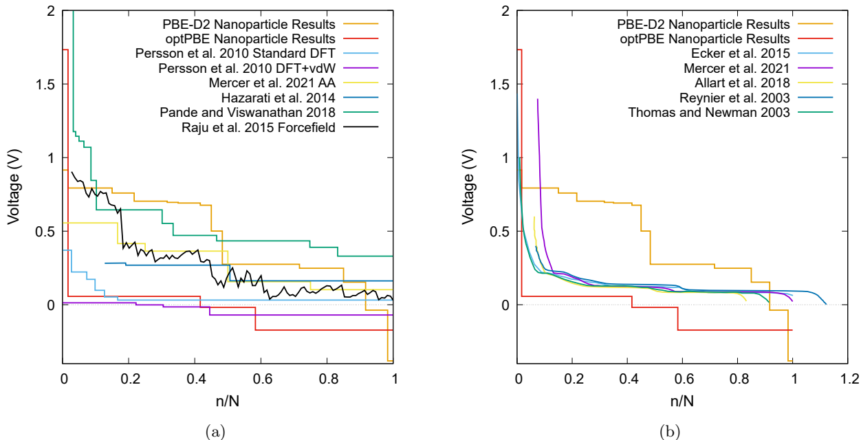
Figure 13: (a) A comparison of computational voltage step profiles with increasing lithiation adapted from references: Persson et al. 18 , Mercer et al. 19 , Hazrati et al. 16 , Pande and Viswanathan 97 , Raju et al. 98 . (b) a comparison of experimentally determined OCVs with increasing lithiation adaption from references: Ecker et al. 99 , Mercer et al. 19 , Allart et al. 27 , Reynier et al. 10 , Thomas and Newman 100 .
