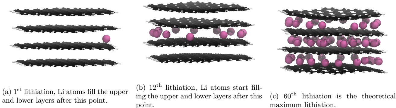
Figure 5: Significant geometry optimised GIC structures from Li intercalation with Li placement restrictions (c.f. 3.5), using the optPBE correction functional. Li atoms are in pink, C atoms in black, and H atoms in white. Images of all structures can be found in our supporting information.
