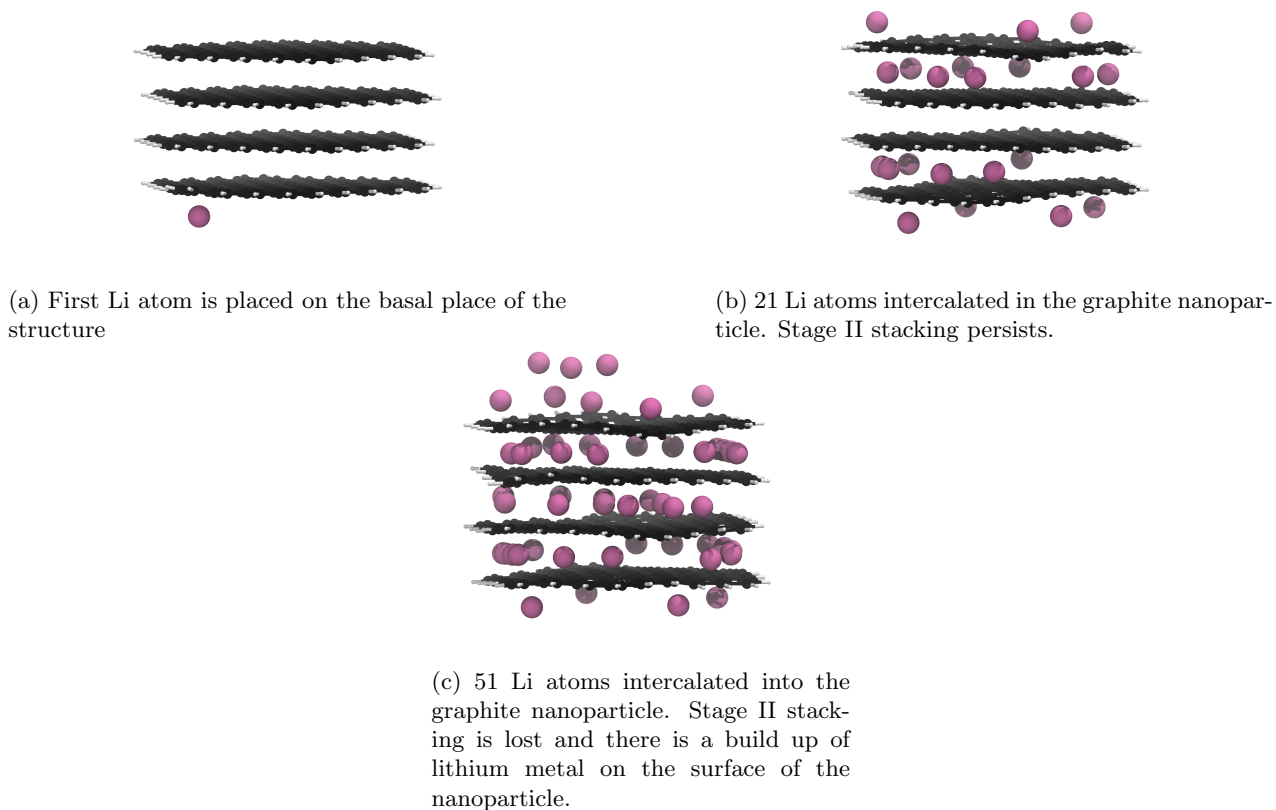
Figure 3: Li intercalation of graphite nanoparticle with unrestricted placement of Li. Li atoms are in pink, C atoms in black, and H atoms in white.
