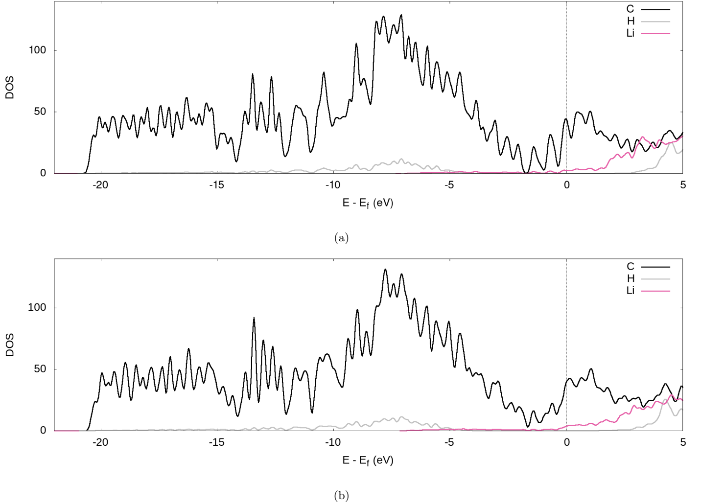
Figure 9: LDOS of the fully lithiated graphite nanoparticle, for our (a) PBE-D2 and (b) optPBE calculations.
