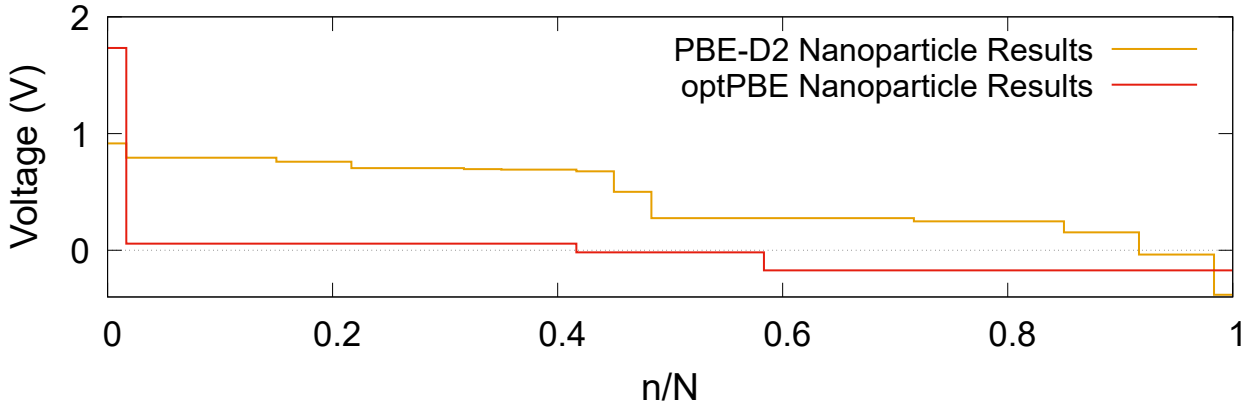
Figure 11: The computed Li intercalation voltage step profiles using two DFT functionals: PBE-D2 and optPBE
