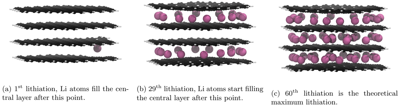
Figure 4: Significant geometry optimised GIC structures from Li intercalation with Li placement restrictions (c.f. 3.5), using PBE with the D2 correction term. Li atoms are in pink, C atoms in black, and H atoms in white. Images of all structures can be found in our supporting information.
