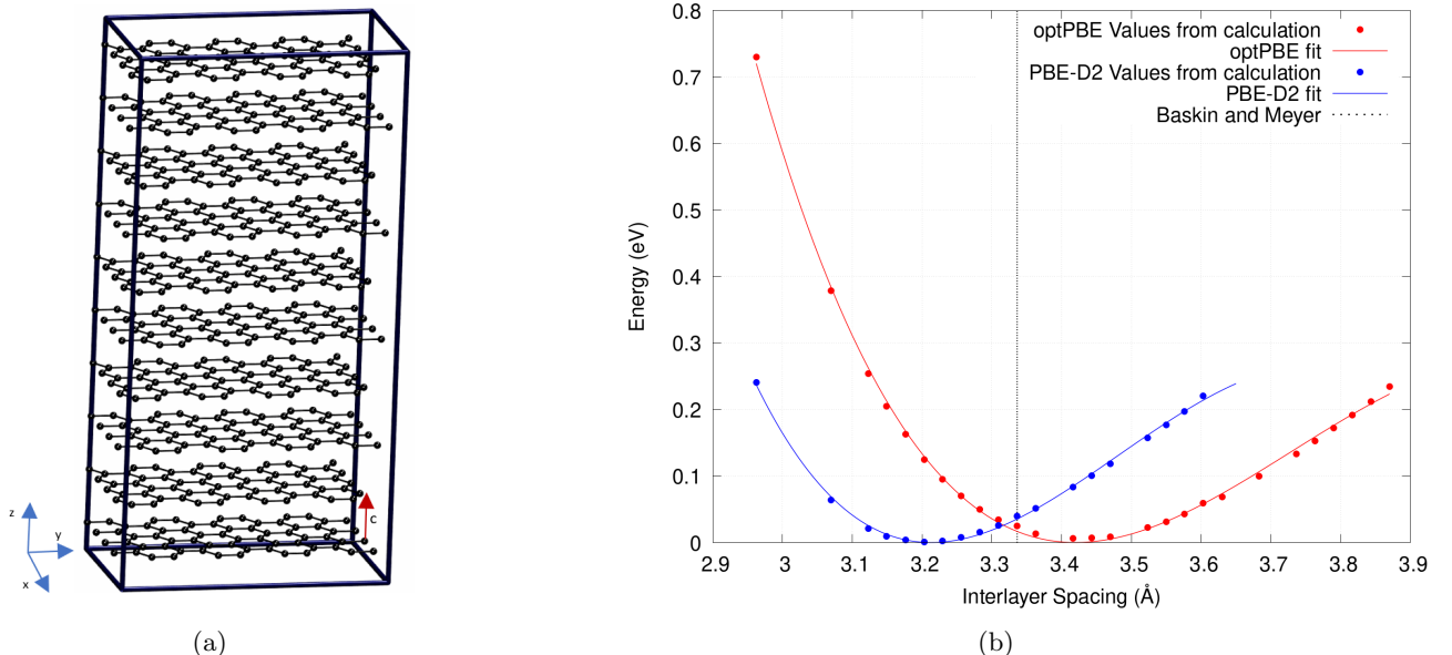
Figure 1: (a) Periodic graphite structure used to test various non-local functionals and empirical correction terms. (b) The relationship between the interlayer spacing of bulk graphite and the total energy. A third-order Birch-Murnaghan equation of state was used to fit this plot. Results of the optPBE non-local functional and PBE with the D2 correction term are shown. 63,65 Experimental results by Baskin and Meyer are also shown. 68
