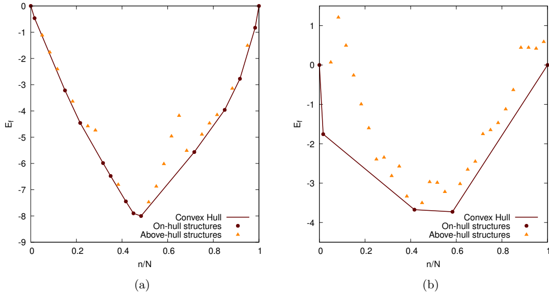
Figure 10: The formation energy of the Li intercalated graphite nanoparticles as a function of the degree of lithiation ( n/N ). N = 60 for our graphite nanoparticle, cf. sec. 3.5 The Li intercalation proceeds via the convex hull (shown as brown line). The points on the convex hull (shown as brown circles) are the ground-states. The structures above the convex hull are shown with yellow triangles. Two different DFT functionals are considered: (a) PBE-D2 and (b) optPBE
