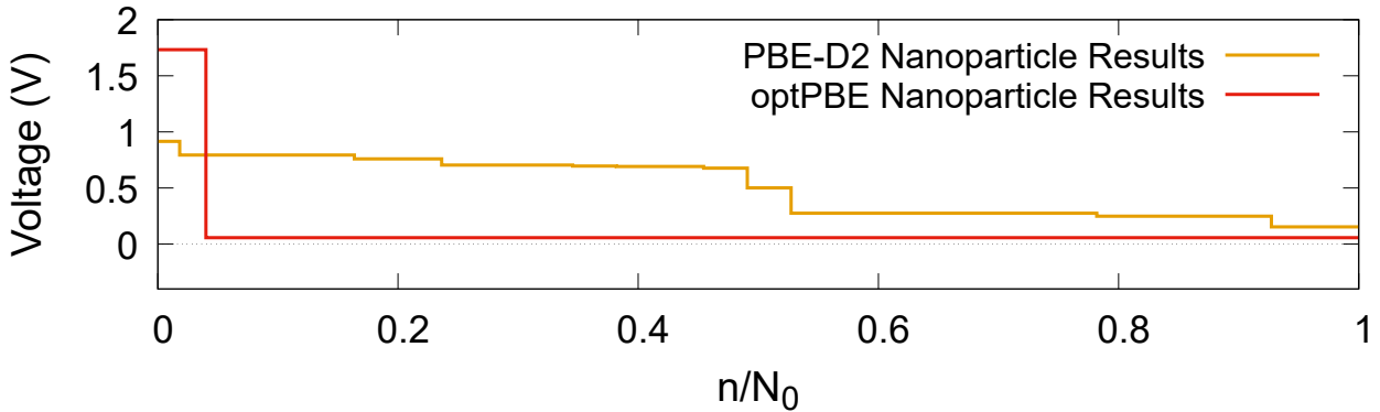
Figure 12: The computed Li intercalation voltage step profiles, where intercalation stops once it becomes thermodynamically unfavourable, using two DFT functionals: PBE-D2 and optPBE
