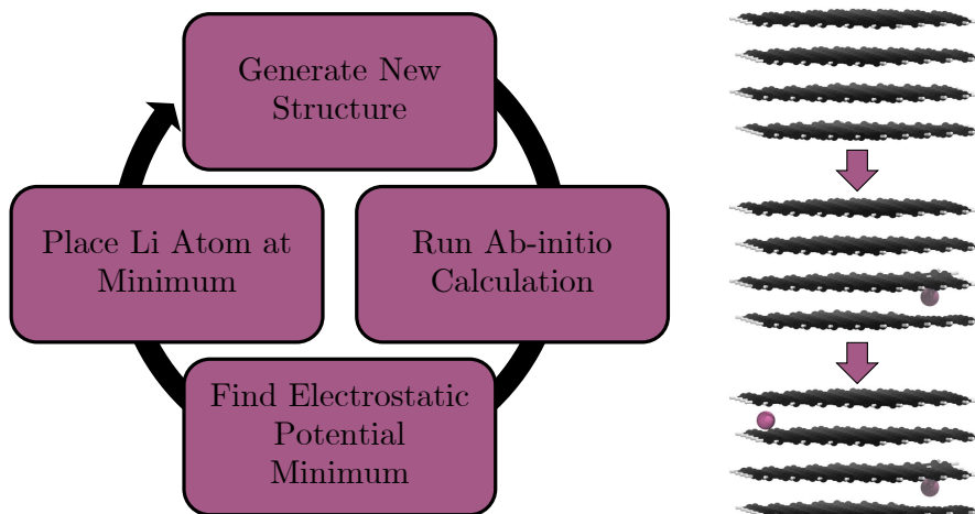
Figure 2: The workflow employed (left) to intercalate a graphite nanoparticle (right) with Li atoms using the electrostatic potential as a guide for Li placement. Li atoms are in pink, C atoms in black, and H atoms in white.
