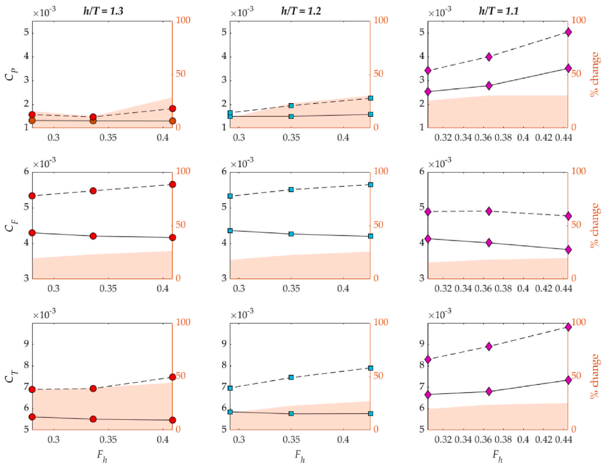
Fig. 5. Comparison of resistance coefficients obtained for a smooth (solid lines) and rough (dashed lines) hull. The axes on the right show the relative change in resistance coefficient.
