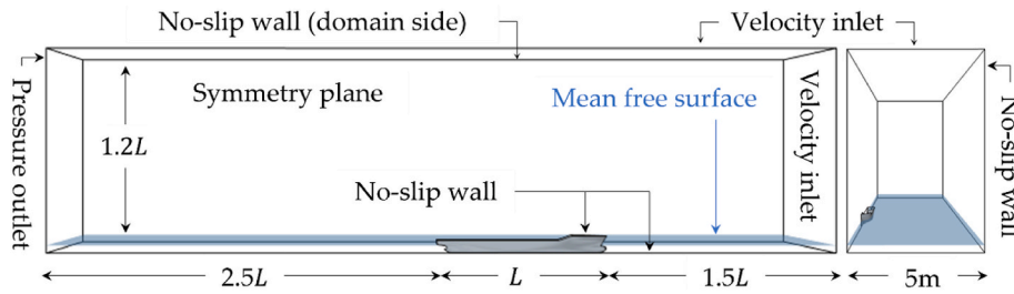
Fig. 1. Graphical depiction of the computational domain and applied boundary conditions. Depicted: h/T = 1.1 .
