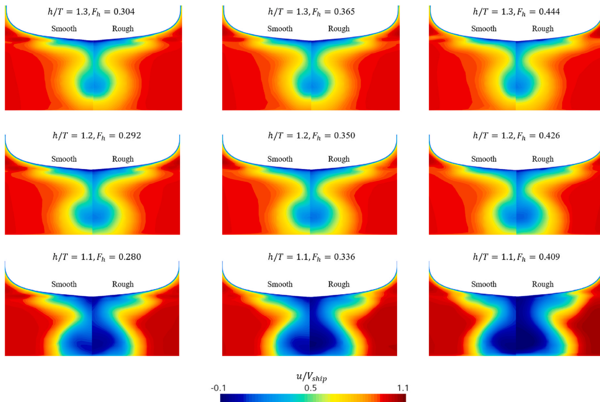
Fig. 10. Wake at the aft perpendicular for all cases.
