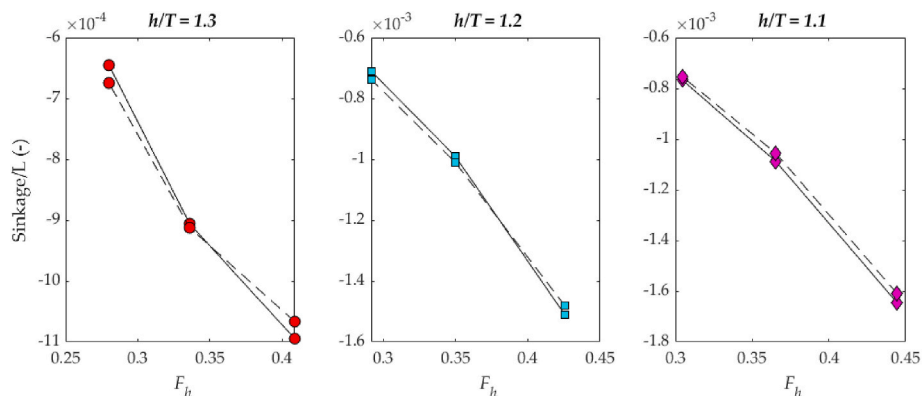
Fig. 8. Sinkage results for smooth (solid lines) and rough (dashed lines) hull conditions.
