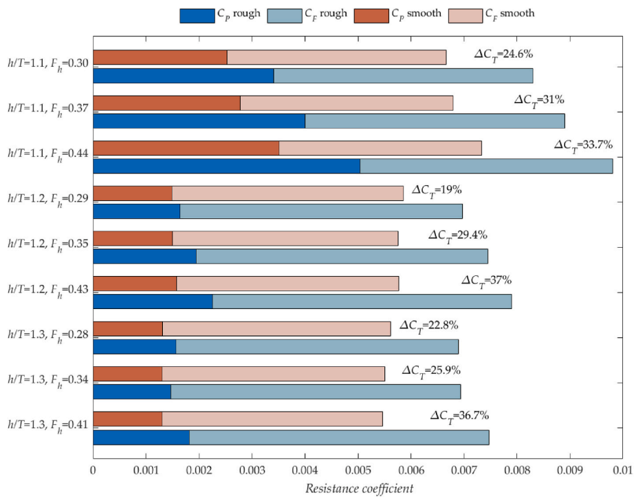
Fig. 6. Total resistance coefficients and relative change due to roughness for all case studies.
