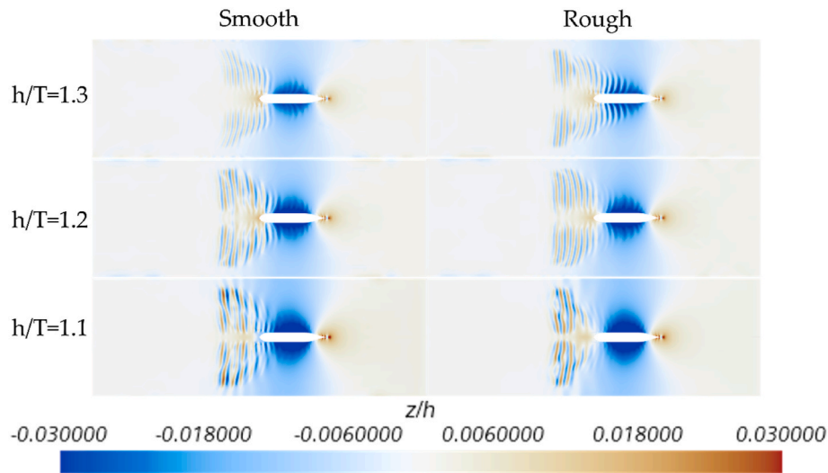
Fig. 11. Wave fields produced by the hull when U = 0.73 m/s.
