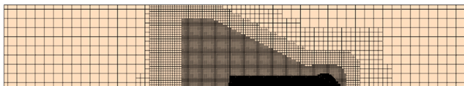
Fig. 3. Top view of the generated mesh on the water surface.
