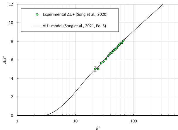
Fig. 2. Experimental roughness function Song et al. (2021) and the roughness function model of Song et al. (2020) (Eq. (5)).
