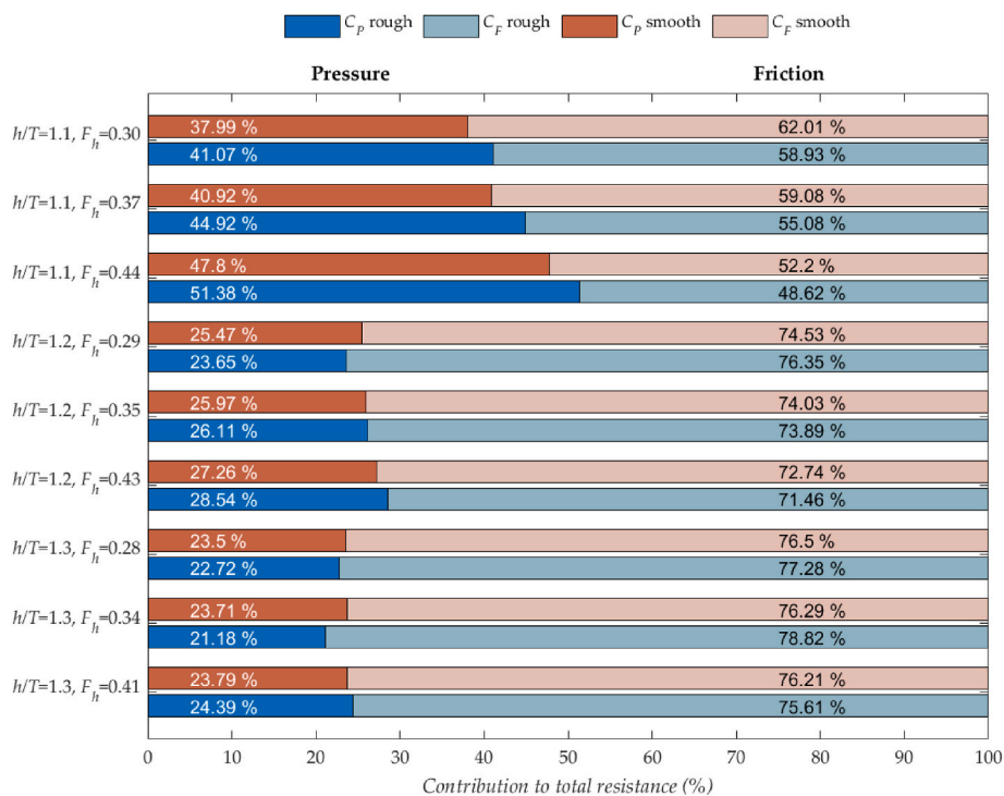
Fig. 7. Make-up of the total resistance coefficient for all case studies.
