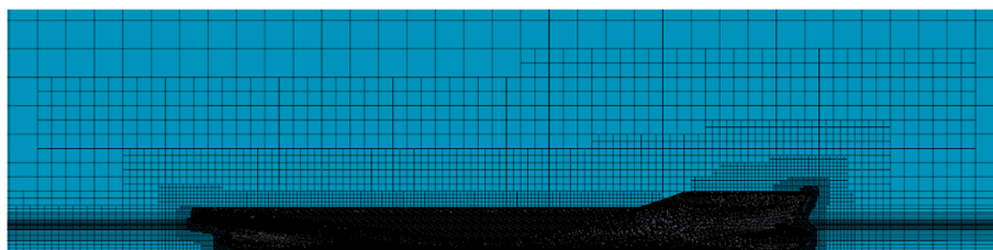
Fig. 4. Close-up side view of the generated mesh on the symmetry plane and the hull. Depicted: h/T = 1.1 .
