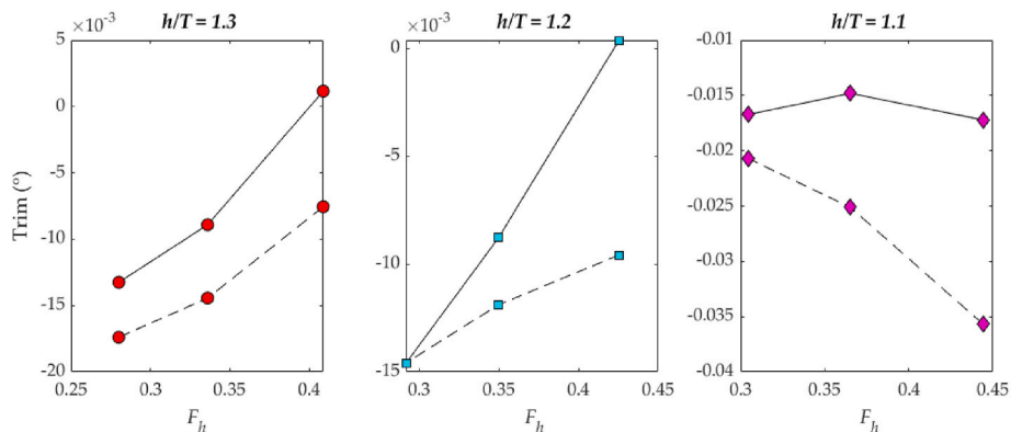
Fig. 9. Trim results for smooth (solid lines) and rough (dashed lines) hull conditions.
