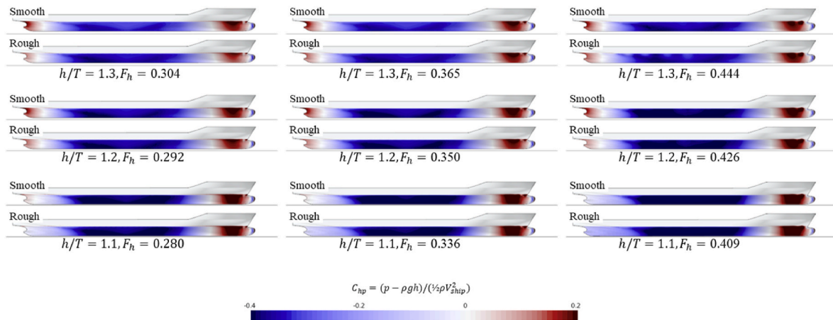
Fig. 12. Hydrodynamic pressure on the hull surface.
