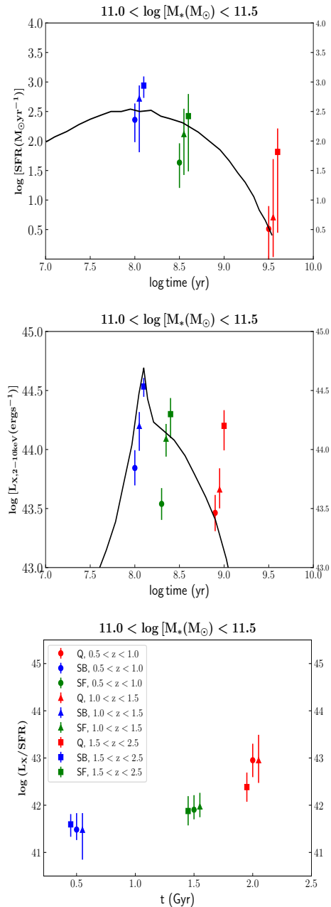
Figure 8. Evolution of SFR (top panel), L_X (middle panel) and their ratio \log L_X/\text{SFR} (bottom panel) with time, for AGN host galaxies with 11.0 < \log [M_*(M_\odot)] < 11.5 . In this exercise, we assume that the galaxy starts its life in a SB phase and then it enters the SF and finally becomes Q. The black lines show the predictions of the model presented in Granato et al. 2004. The x-axis in the top and middle panels, present the galactic age (in log), as shown in Figures 2 and 3 in Granato et al. 2004.
