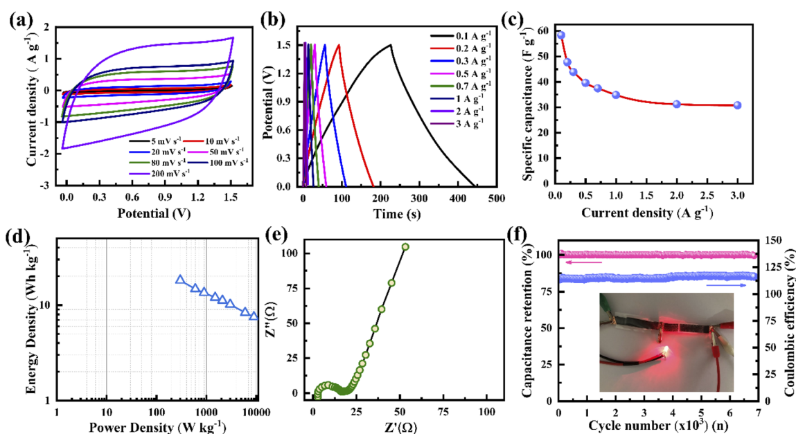
Fig. 7 (a) Cyclic voltammety of the symmetrical supercapacitor with porous graphene electrodes and PVA-KOH-based electrolyte at various scan rates. (b) Galvanostatic charge-discharge of the supercapacitor at various current densities. (c) The specific capacitance of the supercapacitor. (d) Ragone plots of the supercapacitor. (e) Nyquist plots of the supercapacitor. (f) Long cycling performance of the supercapacitor. A light-up LED using the supercapacitor (inset).
