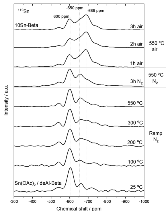
Fig. 9 119 Sn MAS DE CPMG NMR spectra of 10Sn-Beta at different stages of the ramping period in N 2 , and at different stages of the isotherm periods.
