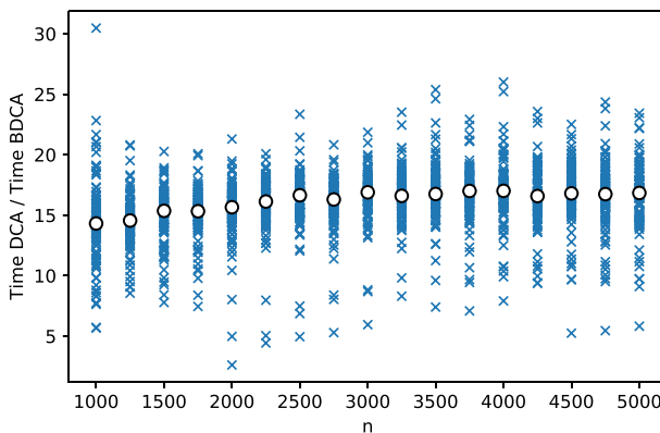
Fig. 1 Comparison between DCA and BDCA for checking the copositivity of Horn matrices of order n \in \{1000, 1250, \dots, 5000\} . For each size, we represent the ratios of the running time between DCA and BDCA for 100 random starting points (blue crosses) and the median ratio among all of them (white circle)
