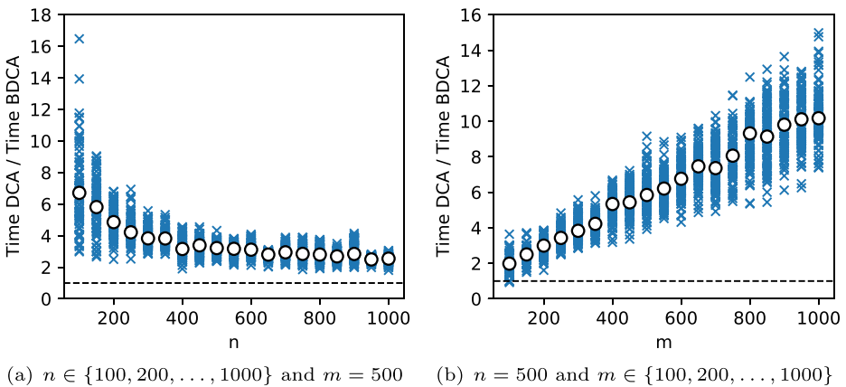
Fig. 10 Comparison between DCA and BDCA for solving randomly generated piecewise quadratic problems with m pieces in \mathbb{R}^n , for n \in \{100, 200, \dots, 1000\} and m = 500 (left), and for n = 500 and m \in \{100, 200, \dots, 1000\} (right). For each problem, we represent the ratios of the running time between DCA and BDCA for 100 random starting points (blue crosses) and the median ratio among all of them (white circle)
