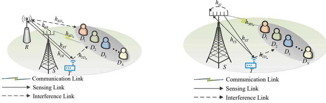
(a): An illustration of the SCC NO-DLT framework. (b): An illustration of the ISAC NO-DLT framework.
