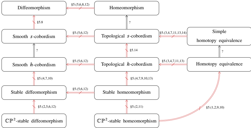
Figure 2. What is known about the converses of the implications in Figure 1. The symbol \nRightarrow denotes the cases where we know an implication does not hold, indicating which subsections contain corresponding counterexamples. The \Rightarrow symbol denotes the three cases where it is unknown whether an implication holds.
