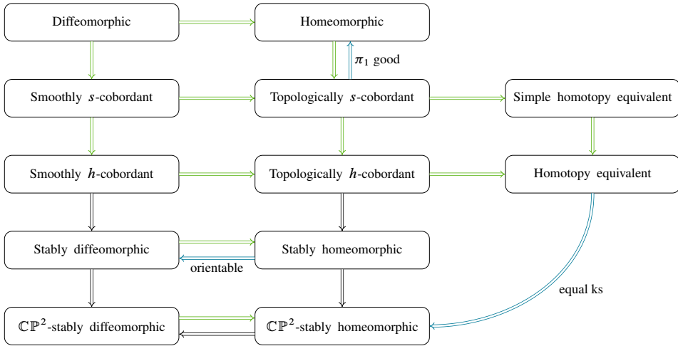
Figure 1. Equivalence relations on 4-manifolds. The implications shown in green are immediate. The black and blue implications are proven in Section 3. The blue implications hold when the corresponding condition is true, e.g. homotopy equivalent 4-manifolds are \mathbb{C}\mathbb{P}^2 -stably homeomorphic if their Kirby–Siebenmann invariants coincide. Where necessary for an implication to make sense, we assume that the manifolds are smooth. For example, the bottom arrow means that closed, smooth \mathbb{C}\mathbb{P}^2 -stably homeomorphic 4-manifolds are \mathbb{C}\mathbb{P}^2 -stably diffeomorphic, since the latter notion is only defined for smooth 4-manifolds.
