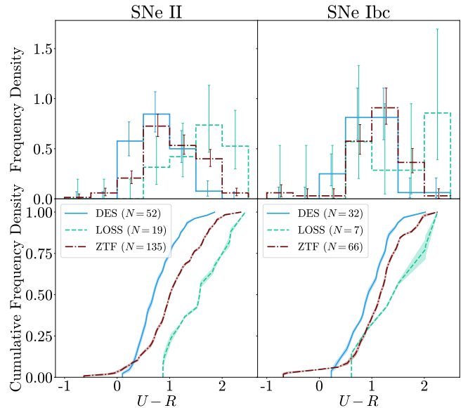
Figure 4. As Fig. 3, but for the host galaxy rest-frame U - R colour in place of stellar mass.
