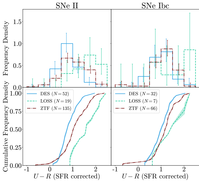
Figure 10. Host galaxy rest-frame U - R colour distributions and cumulative distributions, corrected for the effects of SFR evolution with redshift, for both SNe II and SNe Ibc for DES, LOSS and ZTF samples.
