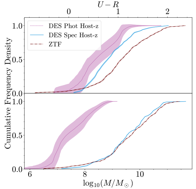
Figure 9. Host galaxy rest-frame U - R (top) and stellar mass (bottom) cumulative distributions for all CCSNe in the the DES sample of objects without spectroscopic host redshifts, compared with the DES sample with spectroscopic host redshifts as well as the ZTF sample.
