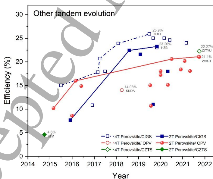
Figure 6- Efficiency evolution for Perovskite-CZTS[1, 2], Perovskite-CIGS[3, 4], and Perovskite-OPV[5, 6] tandem solar cells.
