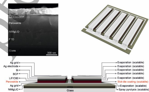
Figure 2 - Interconnection design in perovskite solar modules: a) Series-Connected PSM. Reproduced with the permission of IEEE publisher, b) Parallel-Connected PSM, Reproduced with the permission of Science publisher.
