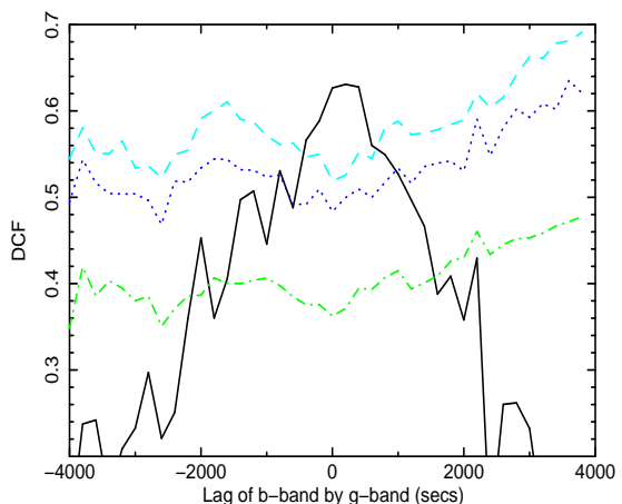
Figure 8. DCF showing the lag of the B-band by the g band in seconds for LT night 2 (Fig. 4). From bottom to top, the 68%, 90% and 95% confidence contours are shown.
