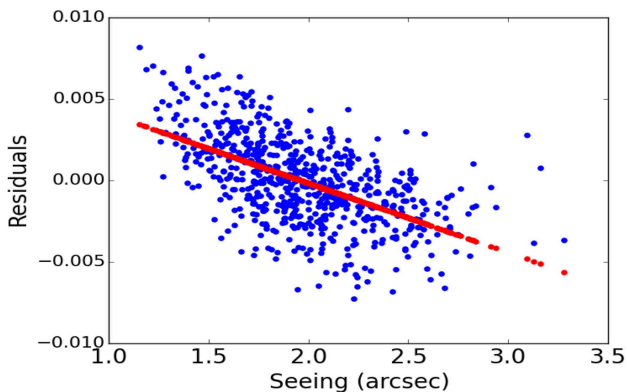
Figure 17. Residuals from Fig 16 vs seeing.
