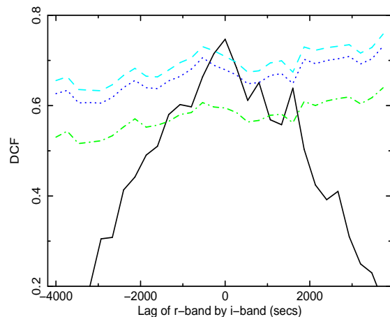
Figure 9. DCF showing the lag of the r band by the i band in seconds for LT night 3 (Fig. 5). From bottom to top, the 68%, 90% and 95% confidence contours are shown.
