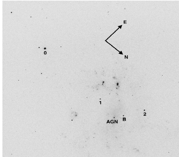
Figure 1. g -band image of NGC 4395, 40s exposure, with the IO:O CCD imager on the Liverpool Telescope. The comparison stars, 0 and 2, used in the production of the LT lightcurves are labelled, as are the comparison stars, 1 and B, used in the production of the HiPERCAM lightcurves. The AGN nucleus is also labelled. The field of view is 10 \times 10 arcmin.
