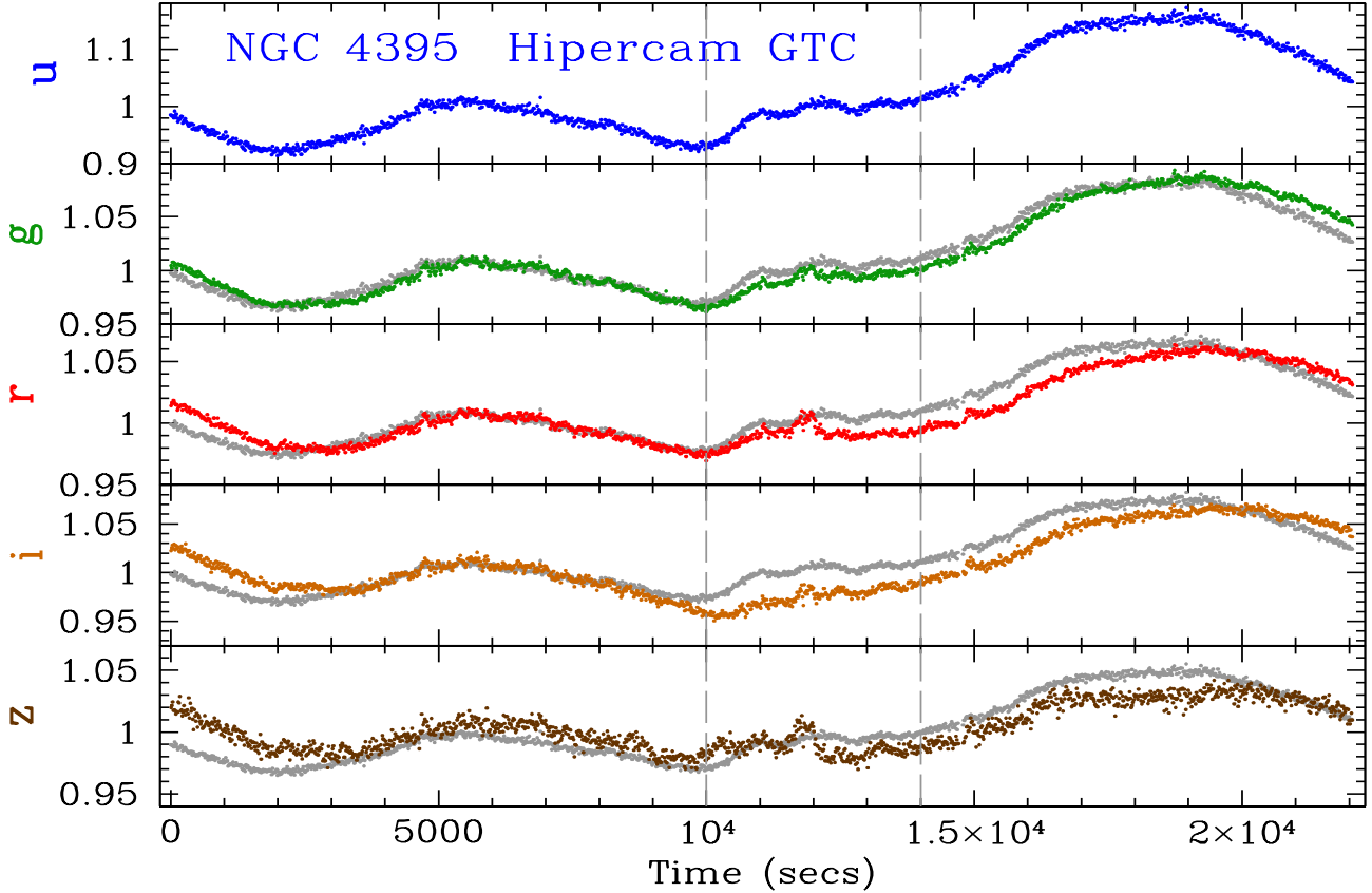
Figure 15. Observed u_s, g_s, r_s, i_s and z_s lightcurves, normalised to the mean, for NGC 4395 from HiPERCAM on the GTC binned to 15s exposures. Statistical errorbars are too small to be seen and are, from u_s to z_s respectively, 0.0047, 0.00165, 0.00175, 0.00243 and 0.00356. The lightcurves between 10,000 and 14,000s, as indicated by the dashed grey lines, are affected by loss of tracking and motion of the target and comparison stars over the CCDs, as described in the text. For each of the g_s to z_s bands, the u_s lightcurve, with variability amplitude scaled to be the same as for the appropriate g_s to z_s band, is underlaid in grey, for comparison.
