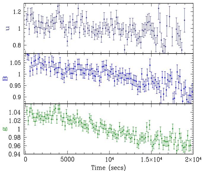
Figure 6. Night 4: As for Fig. 4.
