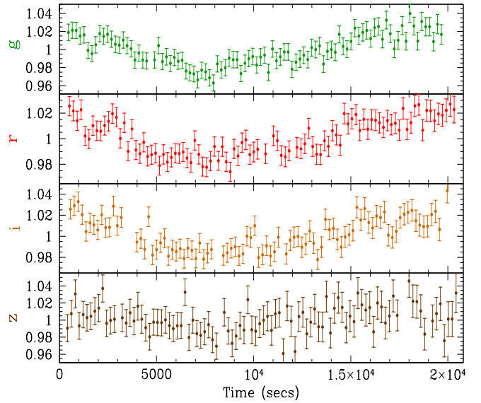
Figure 5. Night 3: As for Fig. 3.
