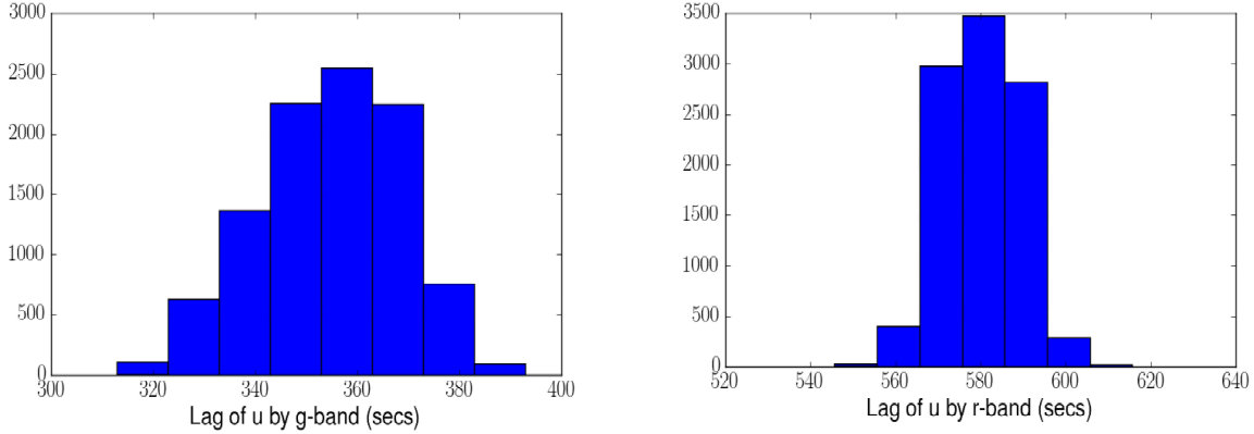
Figure 21. HiPERCAM lag probability distributions from JAVELIN for ( Left ) the g_s , and ( Right ) the r_s , bands relative to the u_s band. The distributions are for the first 8000s of the observation, with lightcurves corrected for seeing changes.
