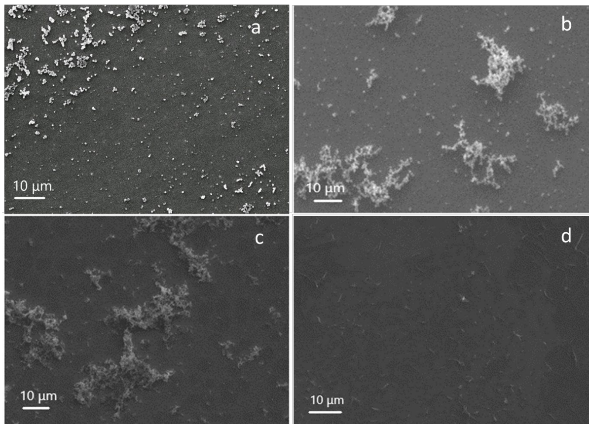
Figure 2. Top view SEM images of EASA films with (a) C 18 TAB, (b) C 18 DMEAB, (c) C 18 DEMAB and (d) C 18 TEAB deposited at an applied potential of -1.25 V (Ag/Ag + ) for 20 s on ITO electrodes.
