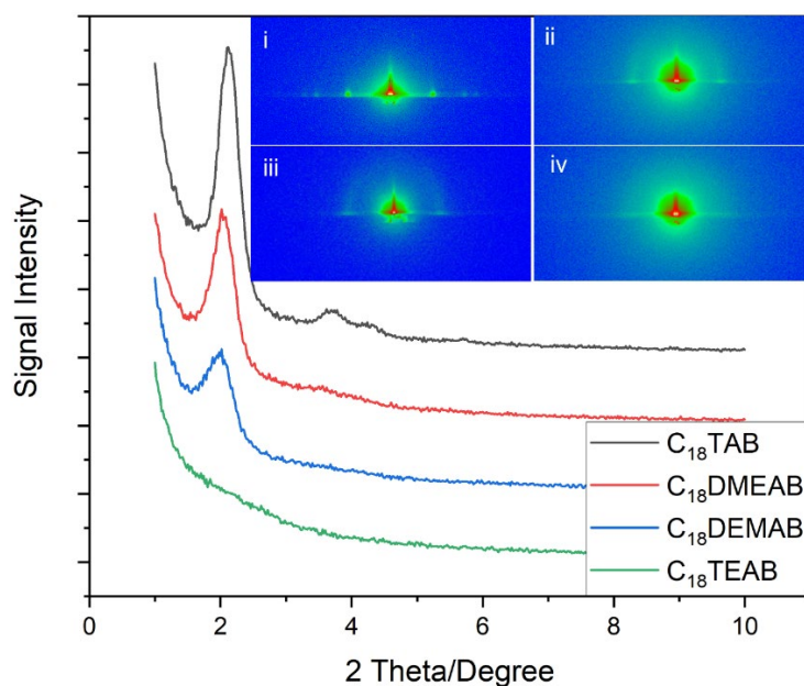
Figure 1. 1D in-plane GISAXS patterns of EASA films produced with C_{18} TAB, C_{18} DMEAB, C_{18} DEMAB and C_{18} TEAB at a potential of -1.25 V (vs. Ag/Ag^+ ) for 20 s on ITO electrodes (inset: 2D GISAXS images of EASA films templated by (i) C_{18} TAB, (ii) C_{18} DMEAB, (iii) C_{18} DEMAB and (iv) C_{18} TEAB).
