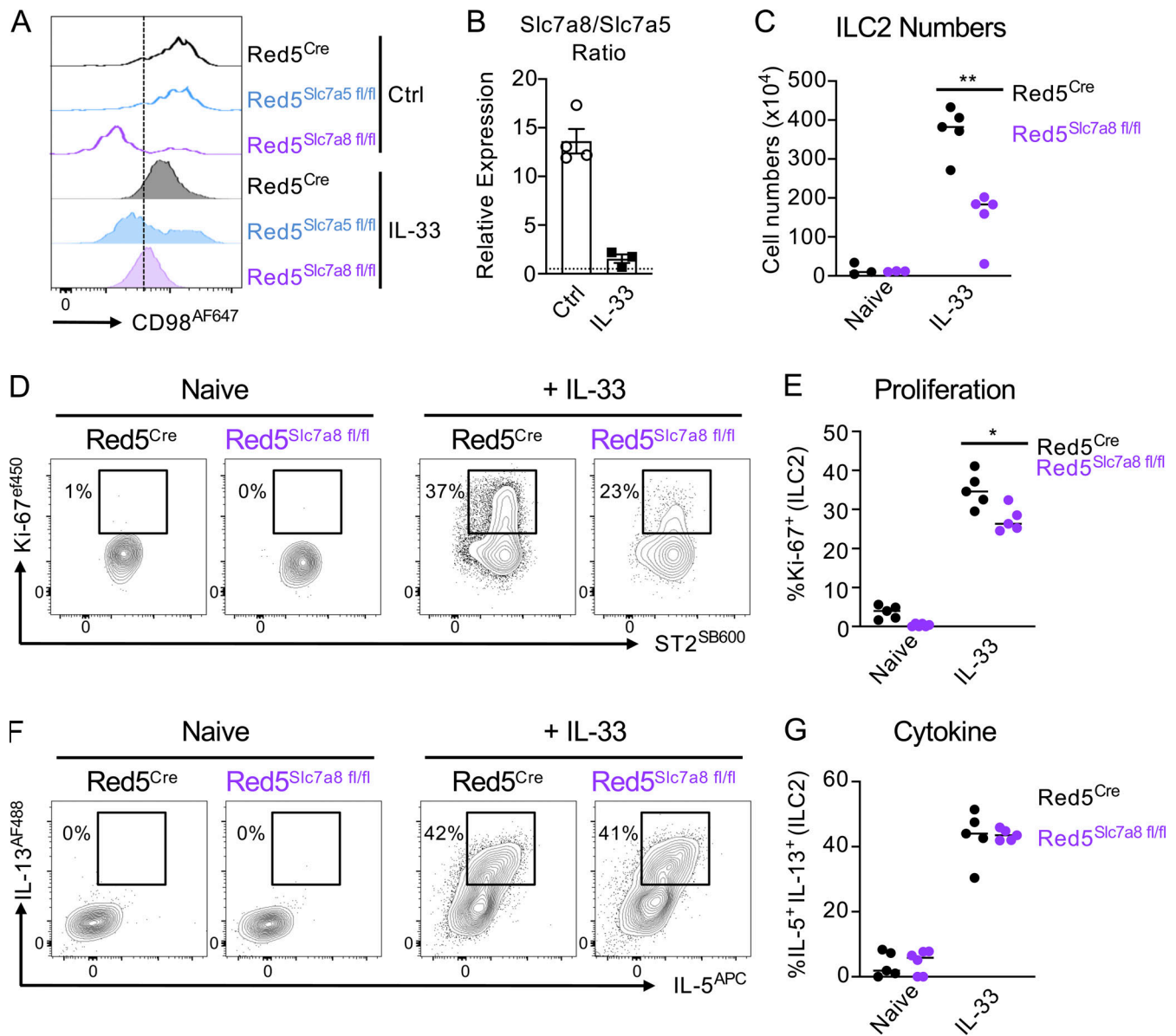
Figure 4. Differential expression of Slc7a8/LAT2 is required for optimal ILC2 expansion following activation. (A) Representative histograms of CD98 expression in lung ILC2 from control (Ctrl) and IL-33-treated Red5 Cre control, Red5 Cre × Slc7a5 fl/fl , and Red5 Cre × Slc7a8 fl/fl mice (representative of n = 3-5 mice per group and at least two independent experiments). (B) Relative expression ratio of Slc7a8 to Slc7a5 in sort-purified ILC2 from control or IL-33-treated animals ( n = 3-4 technical replicates per group, representative of two independent experiments). (C-E) (C) ILC2 numbers, (D) representative flow cytometry plots, and (E) quantification of Ki-67 + ILC2. (F and G) (F) Representative flow cytometry plots and (G) quantification of IL-5 + IL-13 + ILC2 in lung ILC2 from control (Ctrl) and IL-33-treated Red5 Cre control and Red5 Cre × Slc7a8 fl/fl mice. C-G, n = 3-5 mice per group and representative of at least two independent experiments. ILC2 gated as in Fig. S3 A. Data shown as individual values or mean ± SEM. Statistical tests performed: (C and E) one-way ANOVA with multiple comparisons. * P < 0.05 , ** P < 0.01 .
